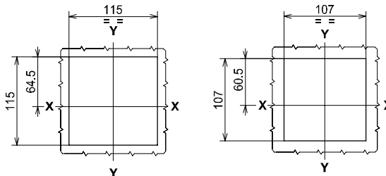
With flange
