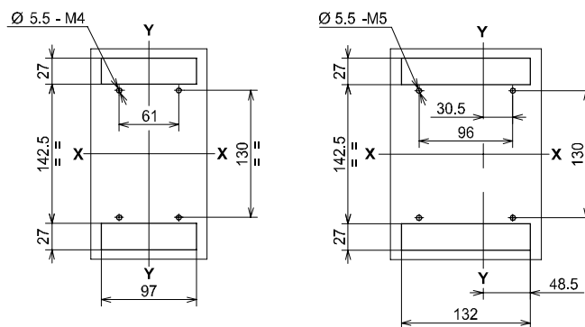
3 POLES
