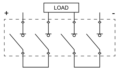
Wiring with jumpers
