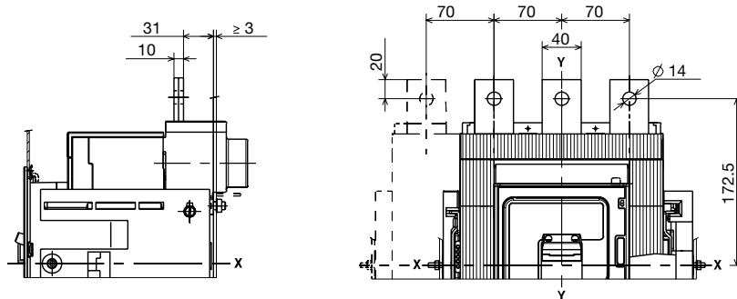
Front extended - EF
