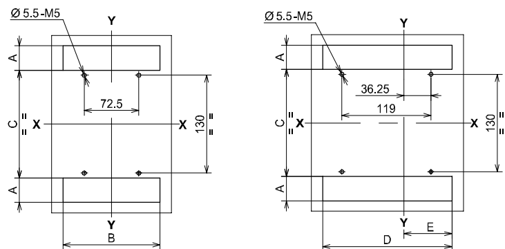
3 POLES
