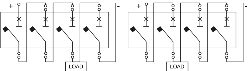
Wiring without jumpers
