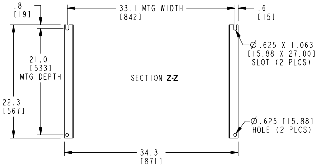
BOTTOM VIEW OF MOUNTING HOLE PATTERN
