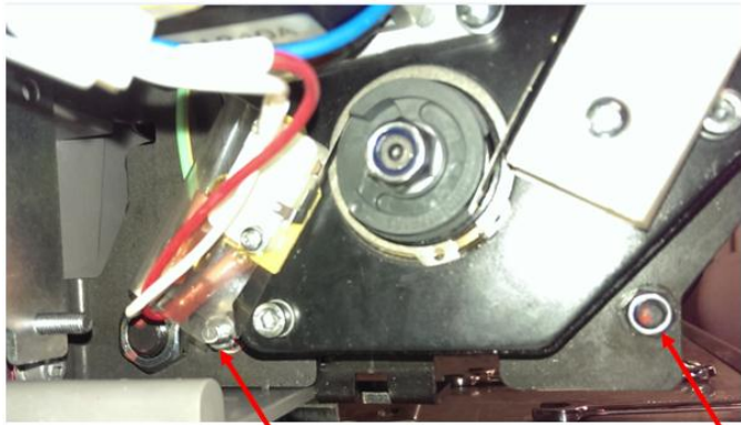
Grounding nut Nylock nut Figure 4.
