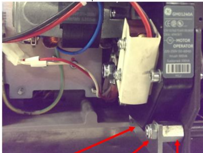
Support bracket Nylock nut Adaptor nut Figure 5.
