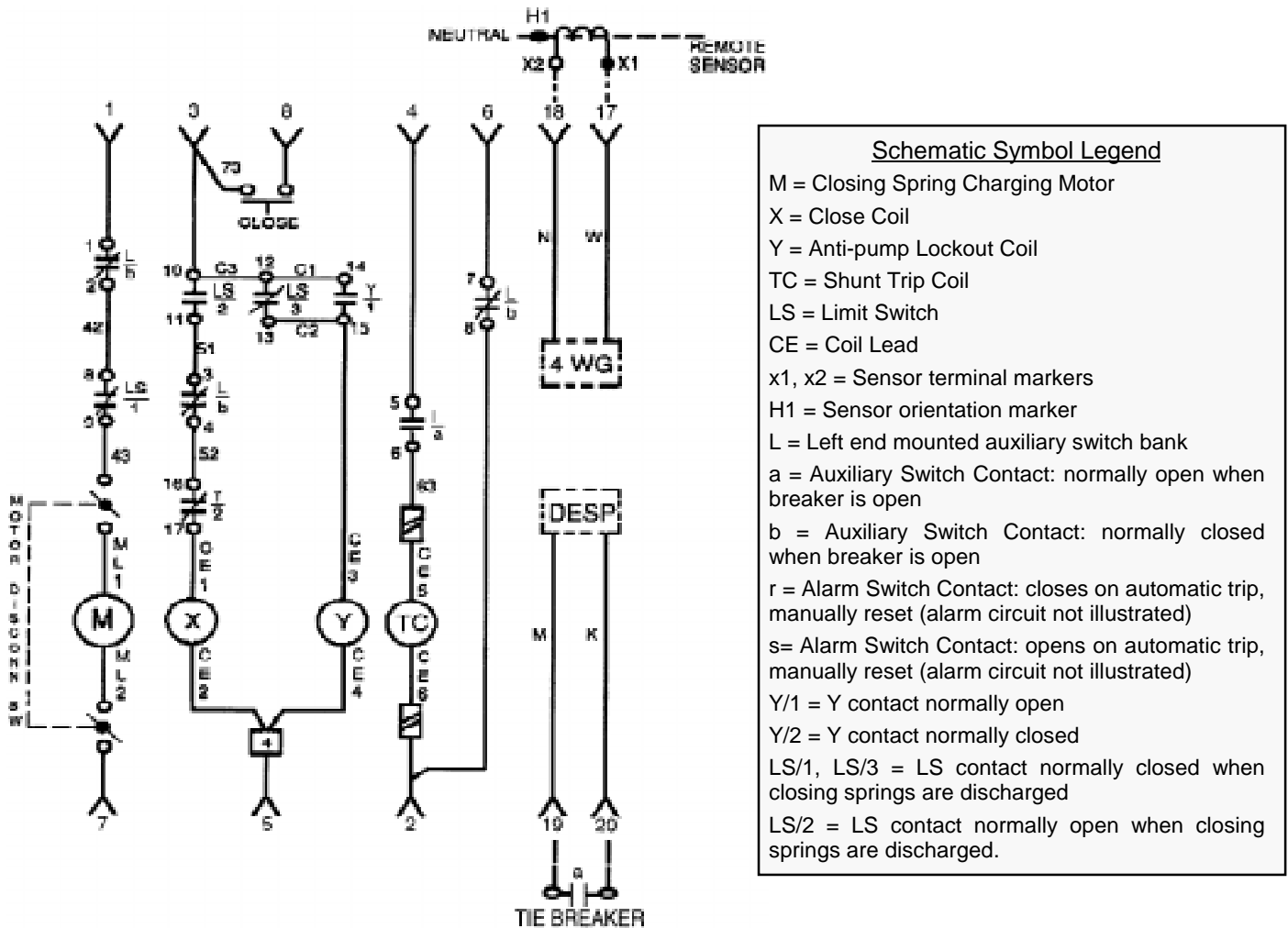
Figure A1. Schematic of a Basic Control Circuit for an EO circuit breaker. Illustrated for a breaker in the OPEN and SPRINGS DISCHARGED state. The basic circuit includes a closing spring charging motor, local electric push button close, control relay device (close and lockout coils), and a shunt trip device. Also shown: optional four wire ground and double-ended substation applications.
