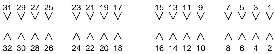
Figure A2. Arrangement of Secondary Disconnects and Contact Identification. Viewed from the rear of the circuit breaker. Depending upon the installed options, a circuit breaker may be equipped with all four pair of secondary disconnects as illustrated.
