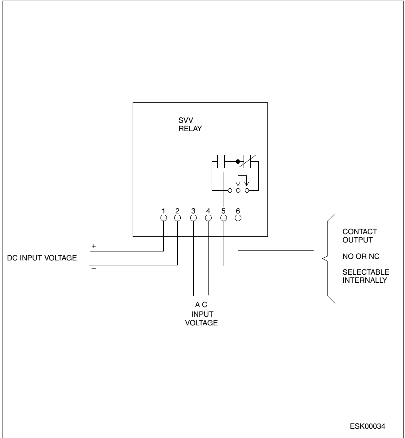
Figure 6. External Connections
