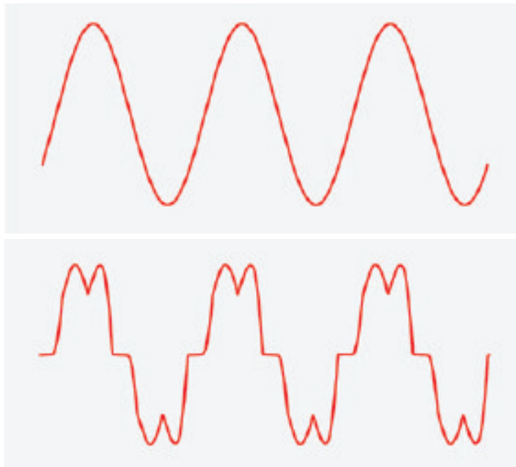
Figure 01 – the ideal electrical supply has a perfectly sinusoidal wave form.
