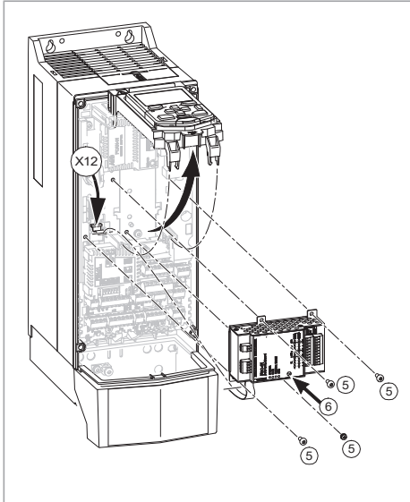
Installation on Slot 2
