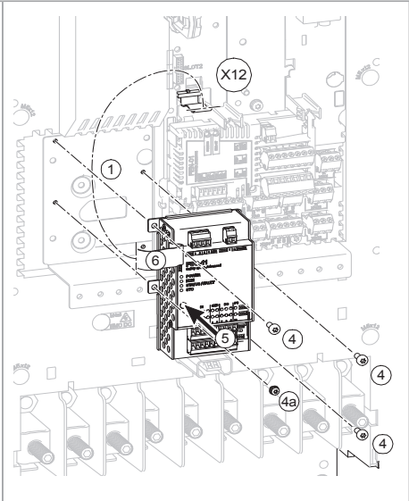
Installation next to the control unit (possible for frames R6...R9)
