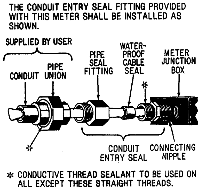
FIGURE 2-9. CONDUIT ENTRY SEAL INSTALLATION
