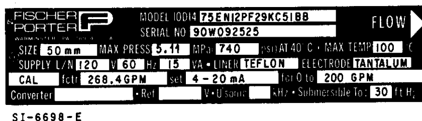
FIGURE 3-1. TYPICAL INSTRUMENT TAG
