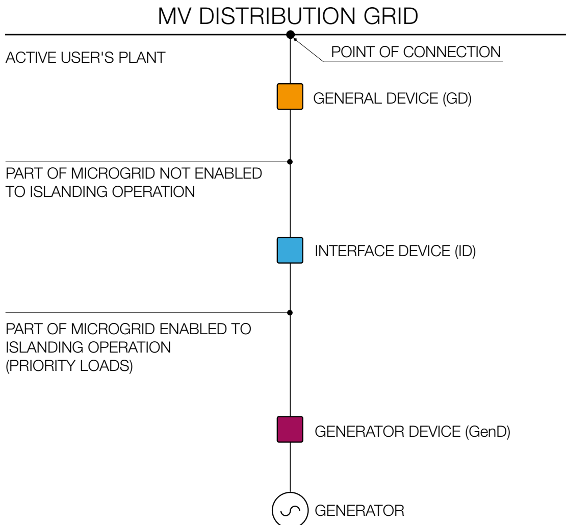
Figure 1 - Typical connection diagram of an Active User
