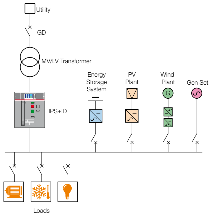
Fig. 3 – Emax 2 as Microgrid Main Circuit-Breaker
