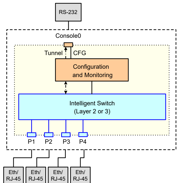
Figure 1: Block diagram of 500NMD50
