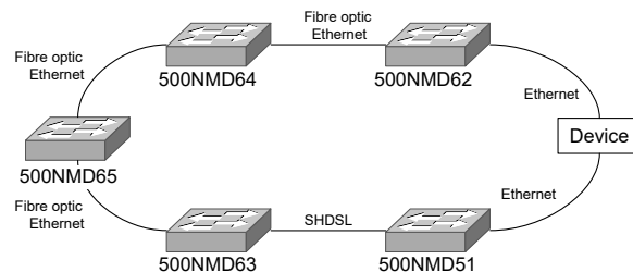
Figure 2: Typical topology for use with 500NMD50
