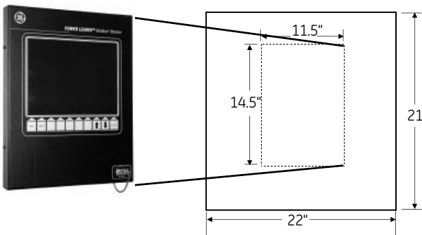
Power Leader Modbus Monitor
