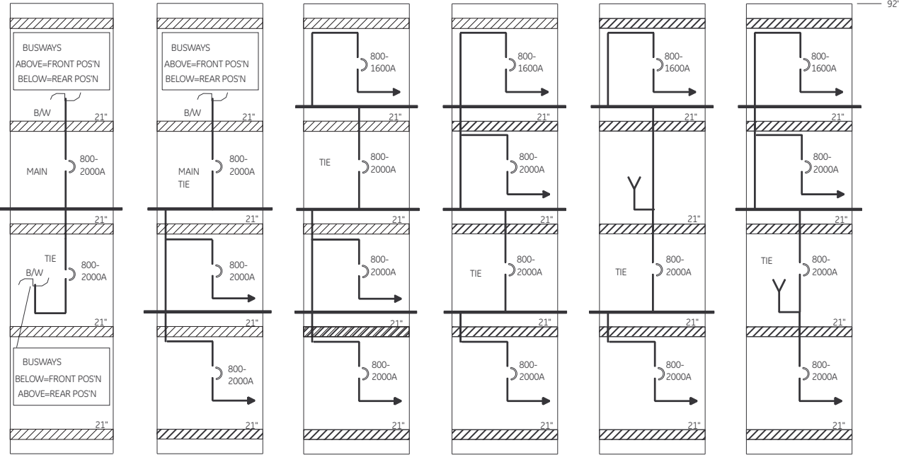
22" MT22-6 MT22-7 MT22-8 MT22-9 MT22-10 MT22-11 30" WIDE WITH 4-WIRE BUSWAY BUSWAY CONN BUSWAY CONN BUSWAY CONN CABLE CONN CABLE CONN MAIN AND TIE MAIN OR TIE TIE TIE TIE TIE
