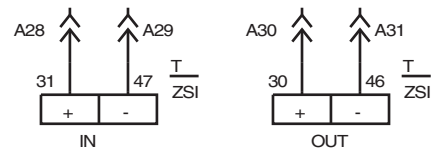
TRIP UNIT ZONE SELECTIVE INTERLOCKING INPUT/OUTPUT (MVT PLUS / PM and "PM READY" ONLY)
