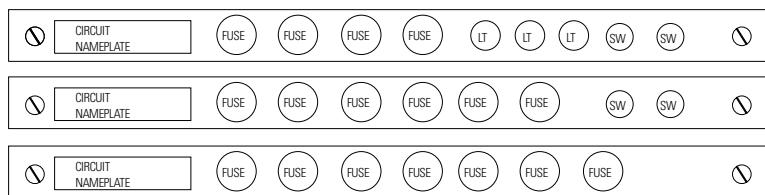
22" WIDE INSTRUMENT PANELS
