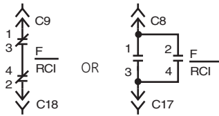
REMOTE CHARGE INDICATOR – NORMALLY OPEN OR CLOSED CONTACT (WPS/H/X-32, WPS/X-40, WPS/X-50 ONLY).
