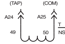
TRIP UNIT NEUTRAL SENSOR INPUT
