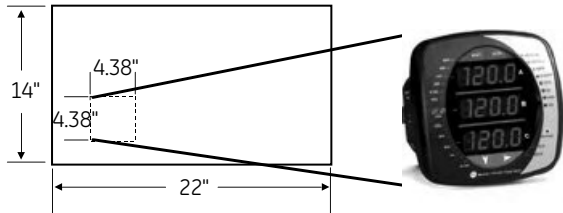
EPM6000 Meter & EPM 9xxx 3-Line Display
