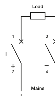
Connection diagram, two-pole (max. 440V d.c.) S402M-UCC
