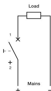
Connection diagram, single-pole (max. 220V d.c.) S401M-UCC
