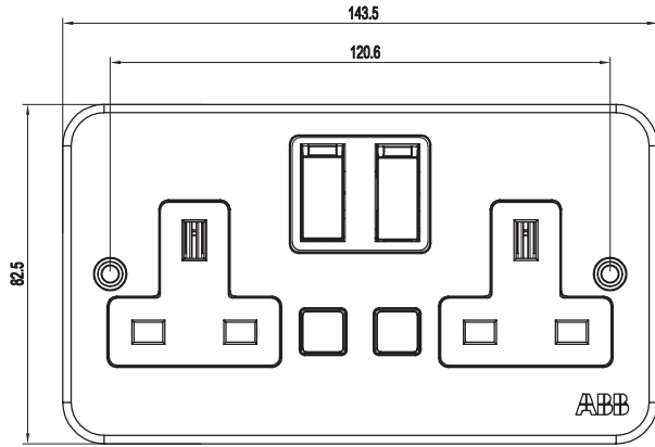
Dimensions for 2 gang frames
