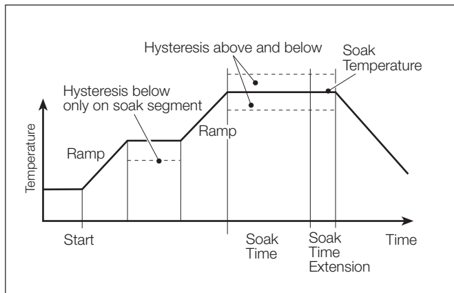
Guaranteed Ramp/Soak
