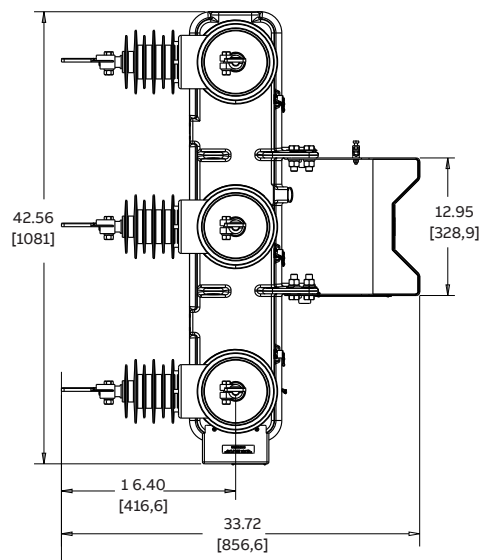
15 kV and 27 kV three-phase reclosers
