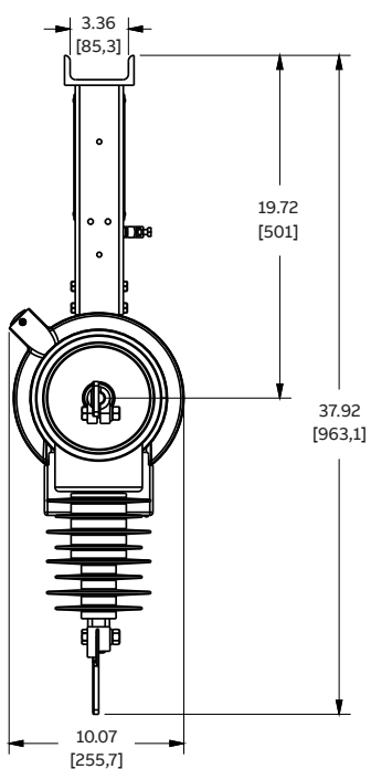
38 kV single-phase recloser
