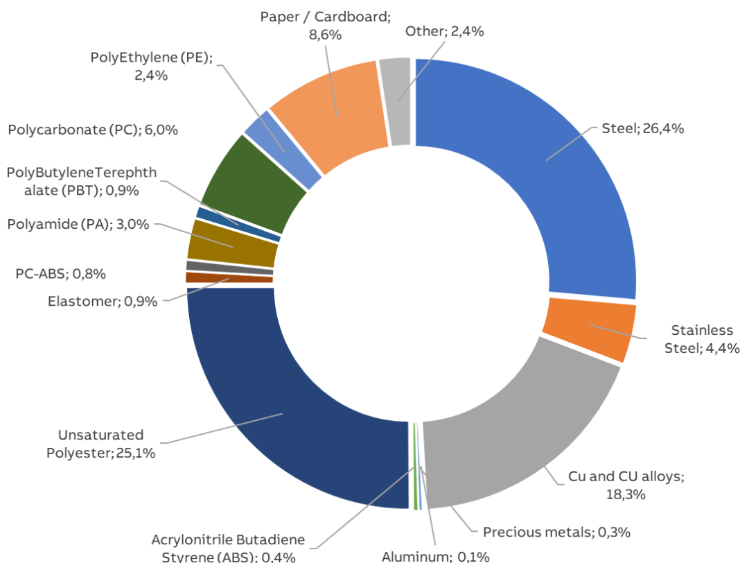
Figure 1: Composition of XT5 3p IEC N/S/H/L Ekip DIP 400A
