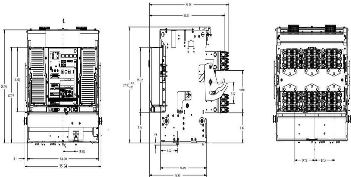
Figure 3A. AKD-10 800-2000A Retrofill Breaker Dimensioning (WPS-50, WPX-50)
