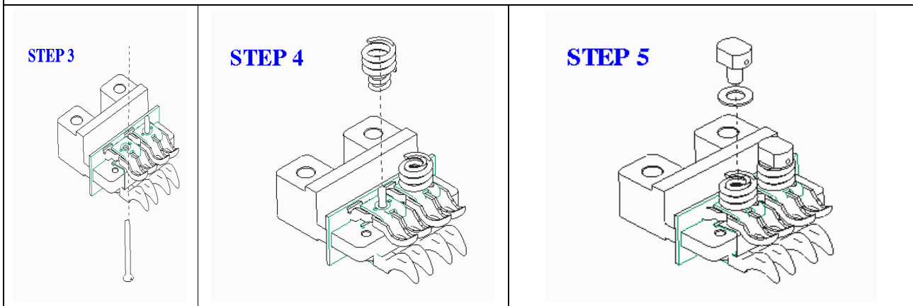
Figure 25. Steps in Exploded Views (WPS-32/WPH-32/WPX-32)
