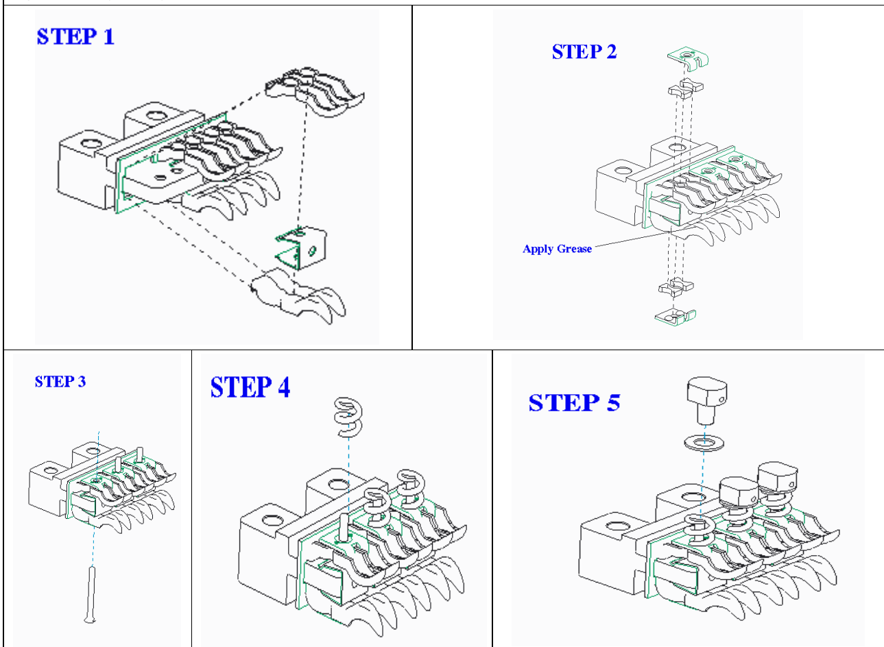
Figure 26. Steps in Exploded Views (A WPS-40/ WPX-40/WPS-50/WPX-50 )
