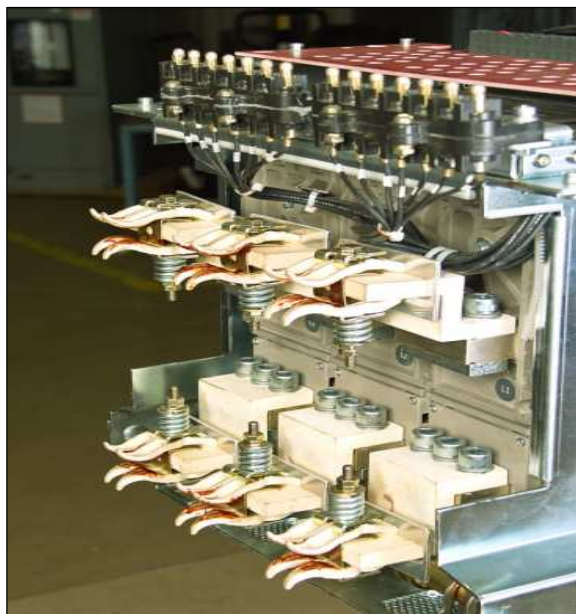
Figure 7. AKD-10—Primary Contacts or “Fingers” (Apply Grease)
