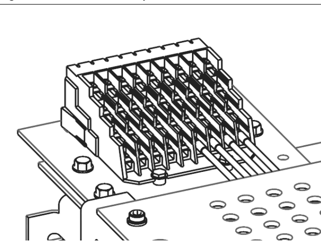
Figure 15. AKD-10 Secondary Disconnects View 2
