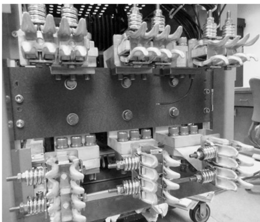
Figure 17. Circuit Breaker Removed, Featuring Primary Disconnects “Fingers” (Contacts)
