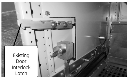
Figure 30A. AKD-10—Door Interlocking Components for WPS-08/ WPH-08/WPX-08/WPS-16/WPH-16/WPS-20 Breaker.
