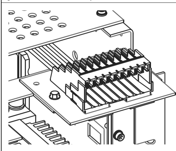
Figure 14. AKD-10 Secondary Disconnects View 1
