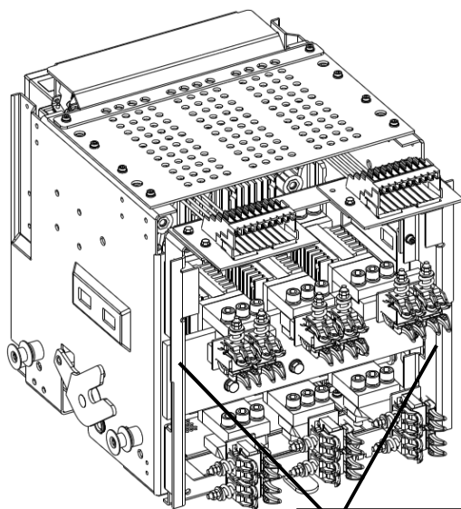
Figure 29. AKD-10—Breaker Surfaces Activate Shutter.
