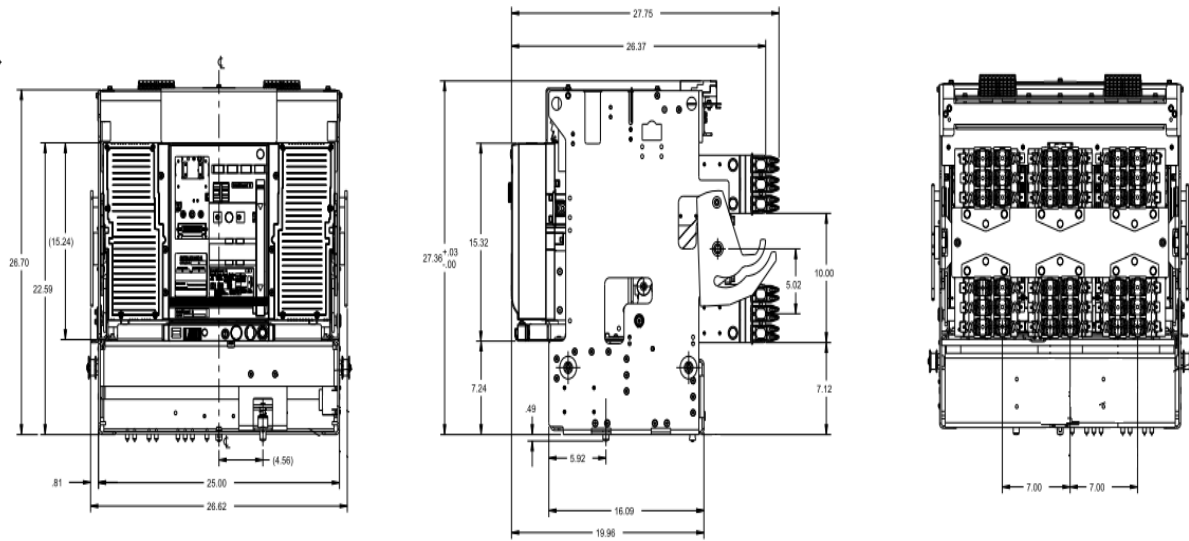
Figure 2A. AKD-10 800A Retrofill Breaker Dimensioning (WPS-32, WPH-32 WPX-32, WPS-40, WPX-40)
