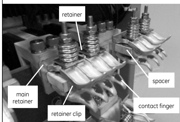
Figure 18. Circuit Breaker, Finger Details
