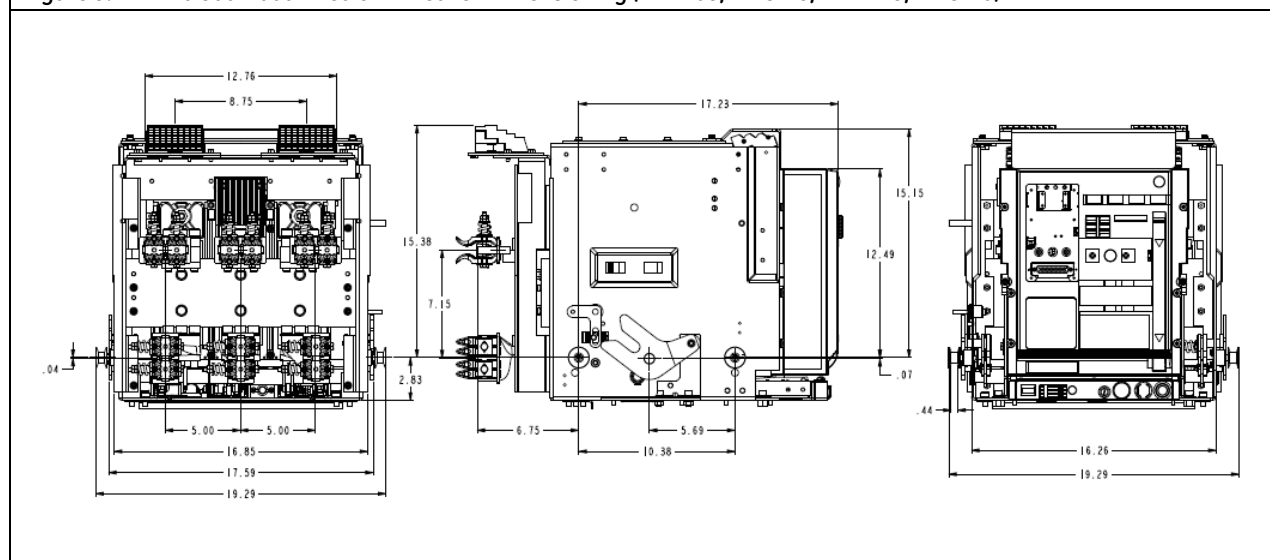
Figure 3. AKD-10 800-2000A Retrofill Breaker Dimensioning (WPX-08, WPS-16, WPH-16, WPS-20)
