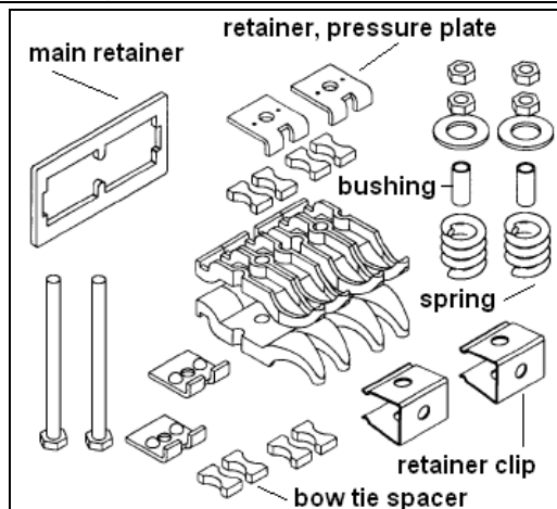
Figure 20. Components
