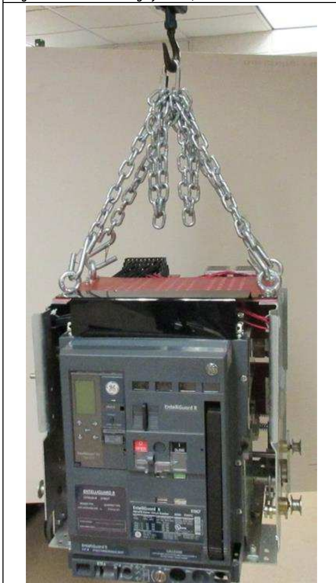
Figure 8D. AKD-10—Using eye bolts, chain and connector.
