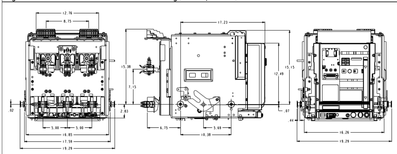
Figure 2. AKD-10 800A Retrofill Breaker Dimensioning (WPS-08, WPH-08)
