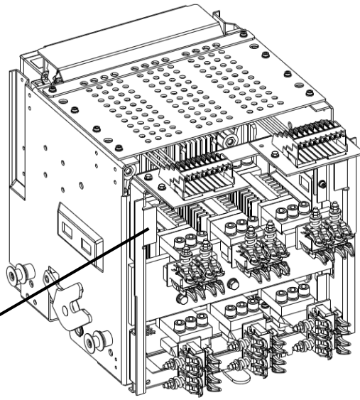
Figure 28. AKD-10 Breaker Surfaces Activate Position Switch.
