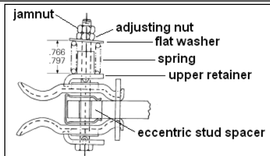
Figure 19. Adjustment
