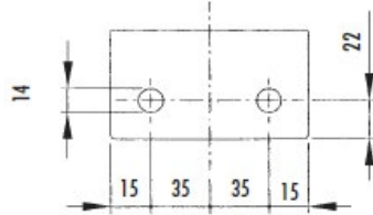
View B (Bracket available for types 7-8)
