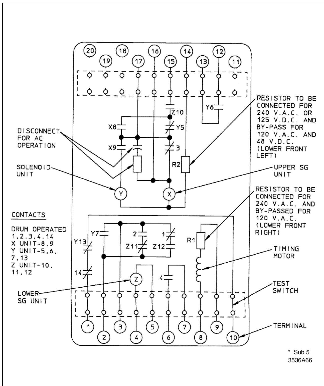
Figure 3. Internal Schematic of the RC Relay, with Z Unit, in Type FT-32 Case
