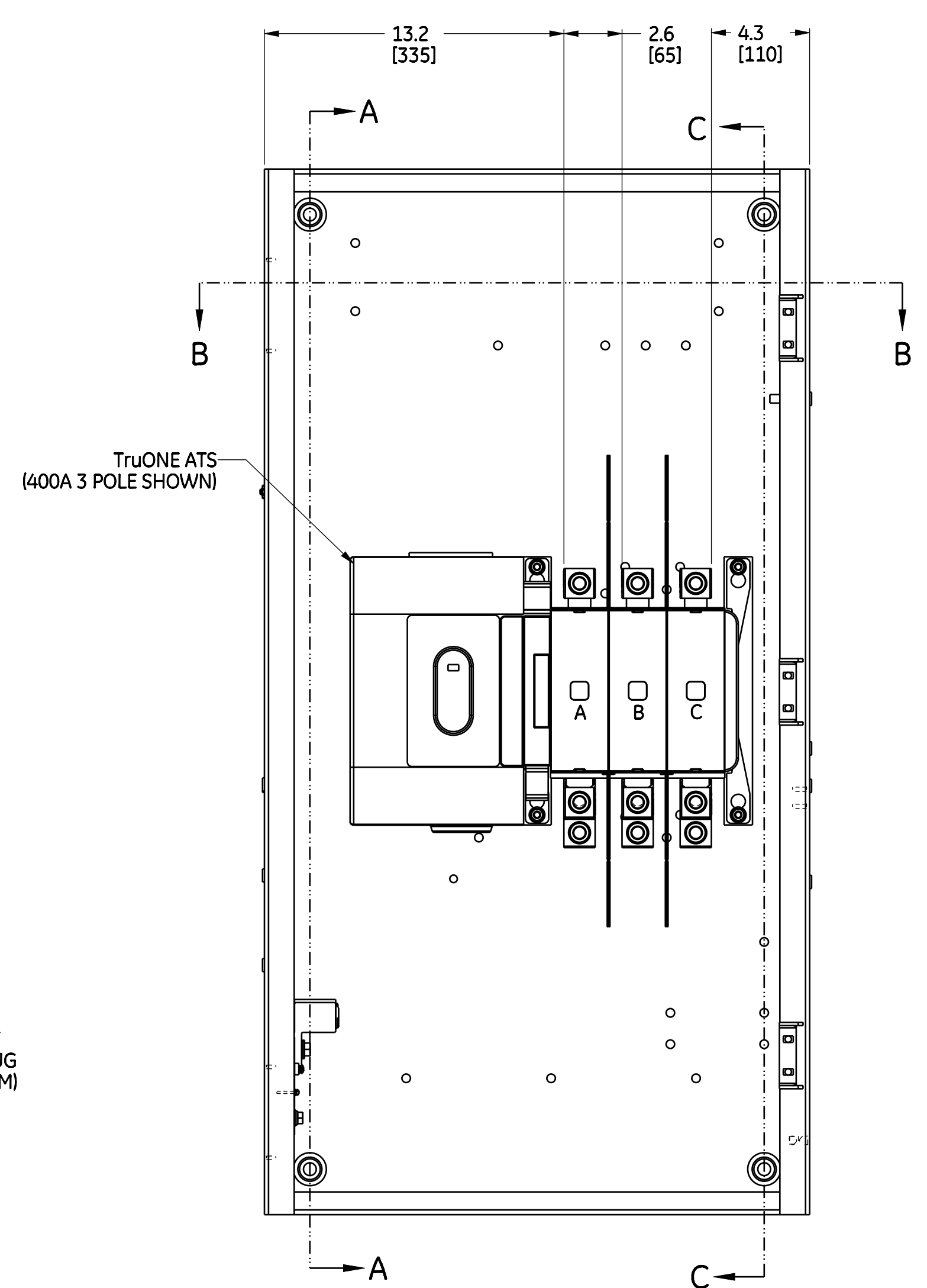
FRONT VIEW WITHOUT DOOR
