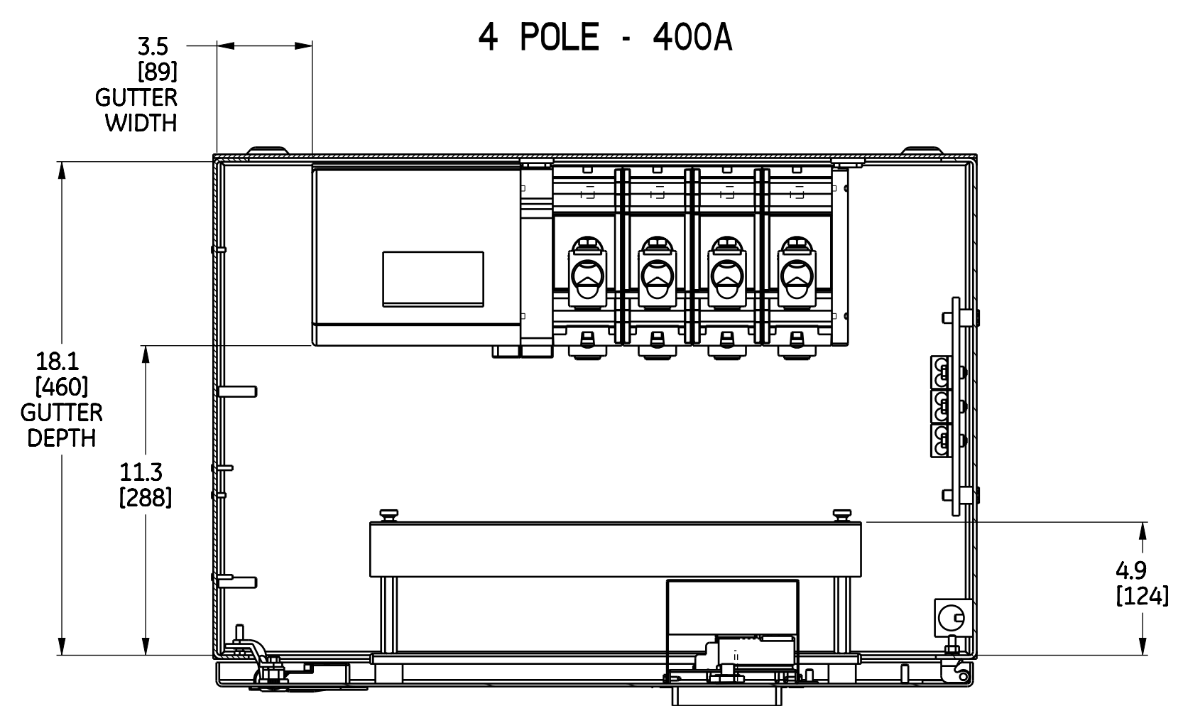
SECTION B-B TOP VIEW WITHOUT TOP PANEL
