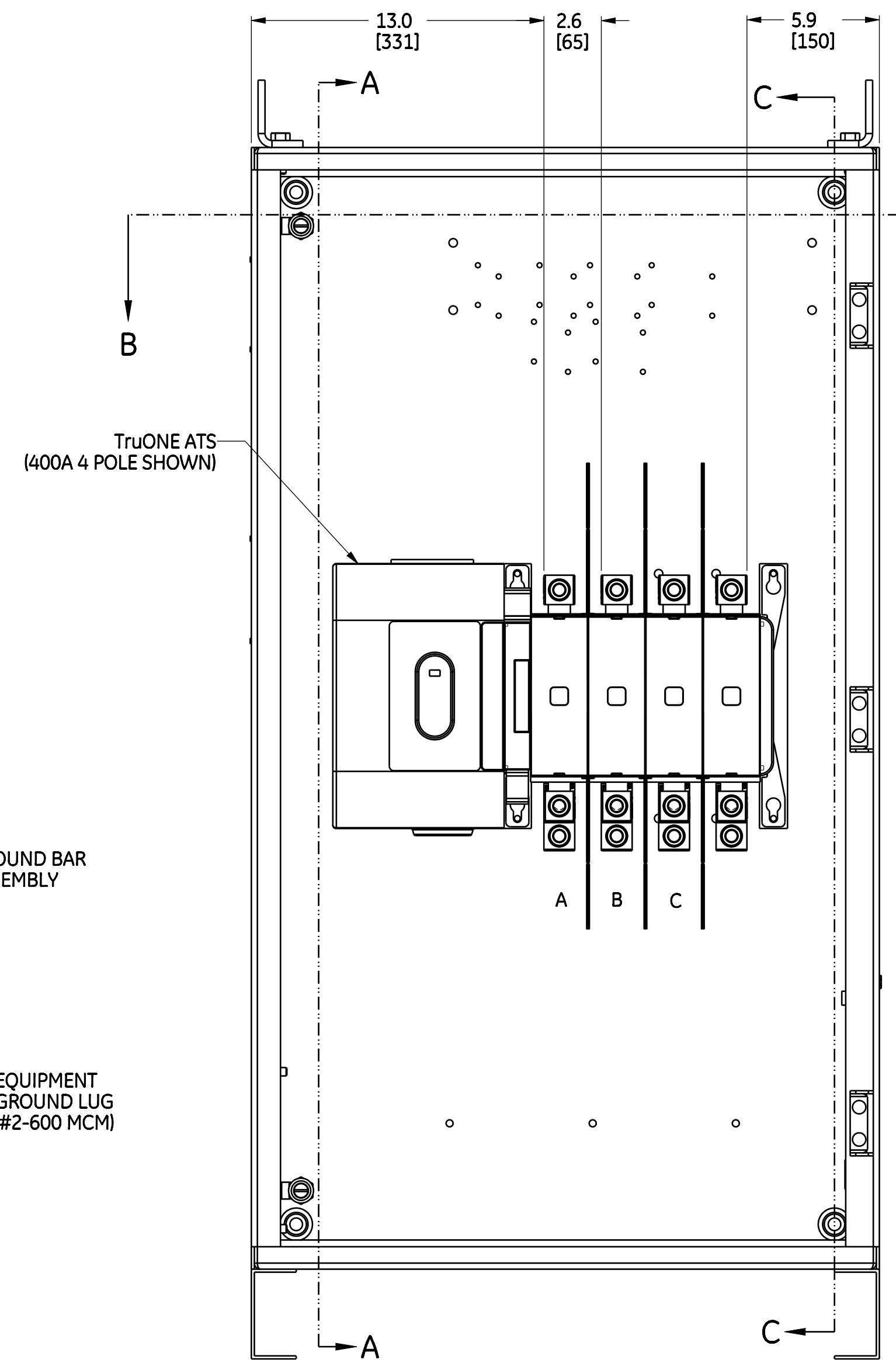
FRONT VIEW WITHOUT DOOR
