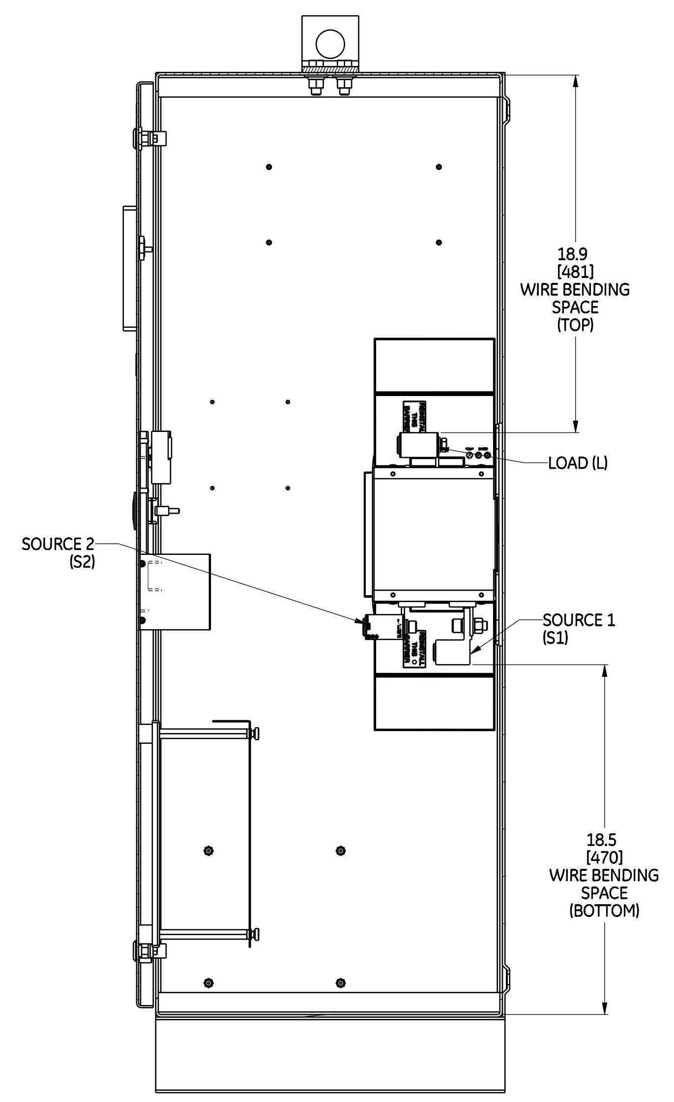
SECTION C-C LEFT SIDE WITHOUT SIDE PANEL
