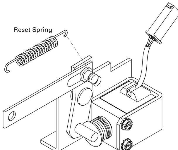
Figure 23. Flux Shifter.
