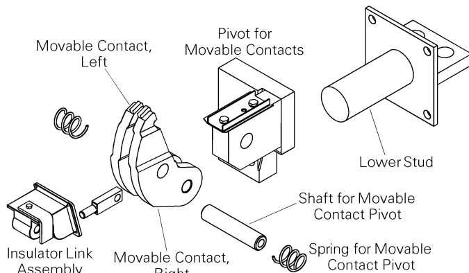
Figure 10. Lower Contact assembly for WPF16, WPS16, WPF16 with 2000 A max fuse and 1200 A max frame current.)
