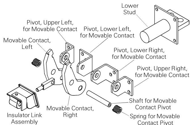
Figure 12. Lower Contact assembly for WPF16 and WPS20. (WPF16 with 2500 A fuse and 1600 A max frame current.)
