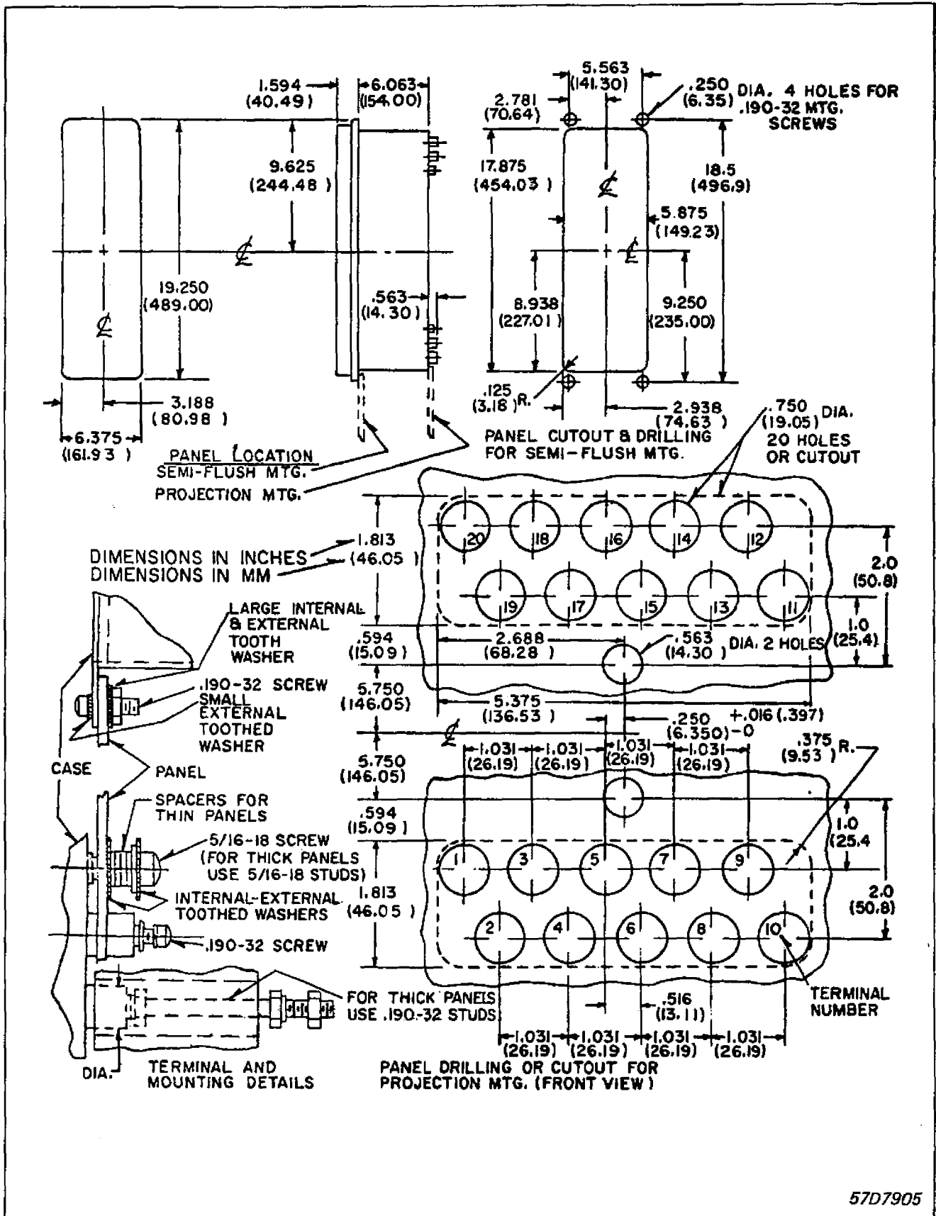
Fig. 7. Outline-Drilling Plan for the Type KDTG Relay in the FT-42 Case.
