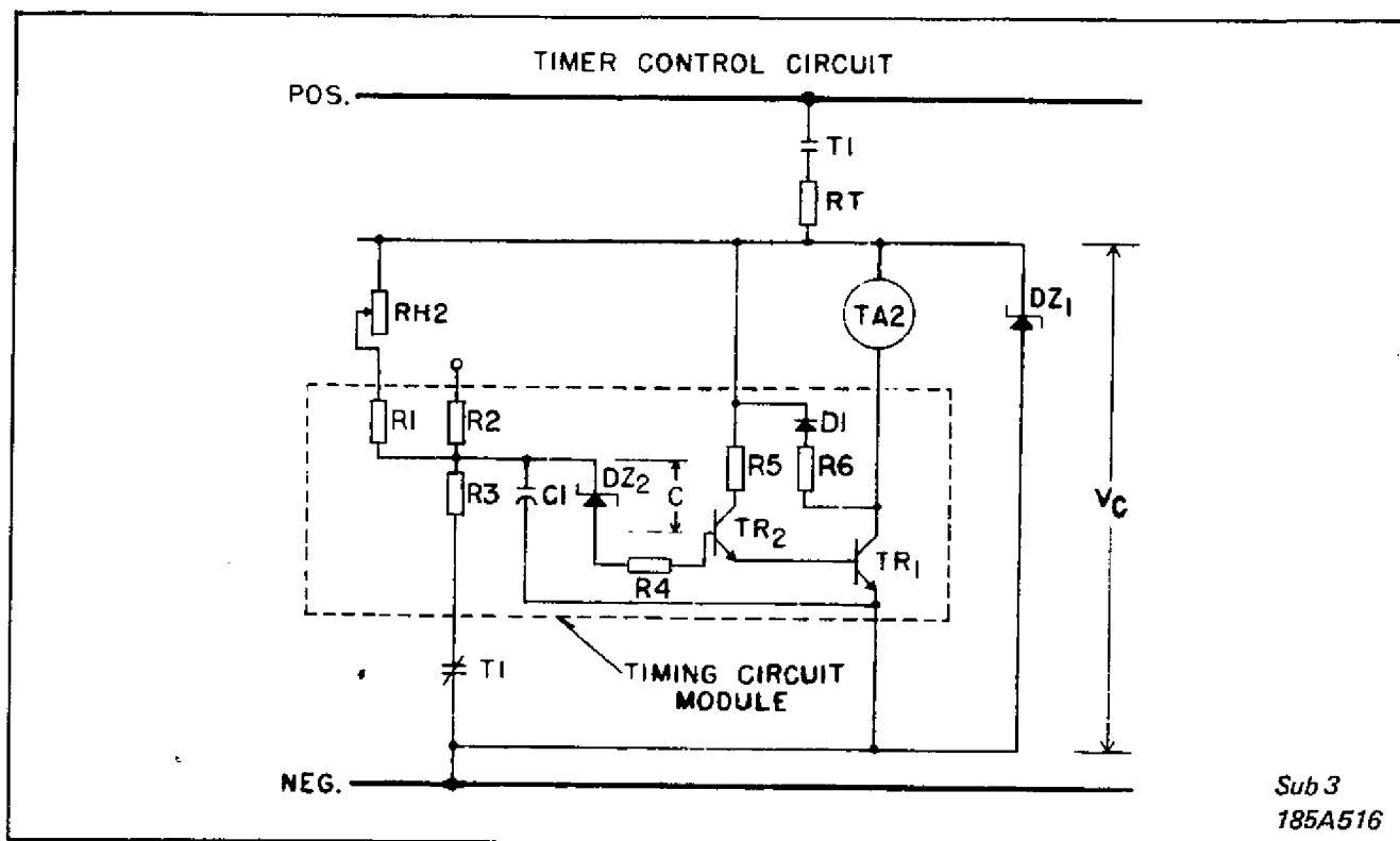
Fig. 3. Module Schematic of the Type KDTG Relay.
