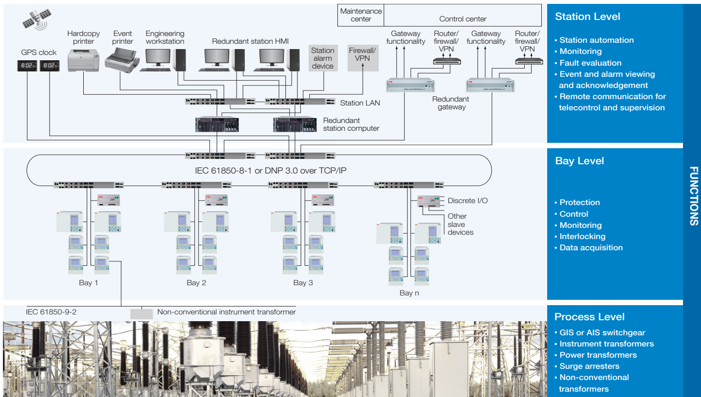
IEC 61850 architecture
