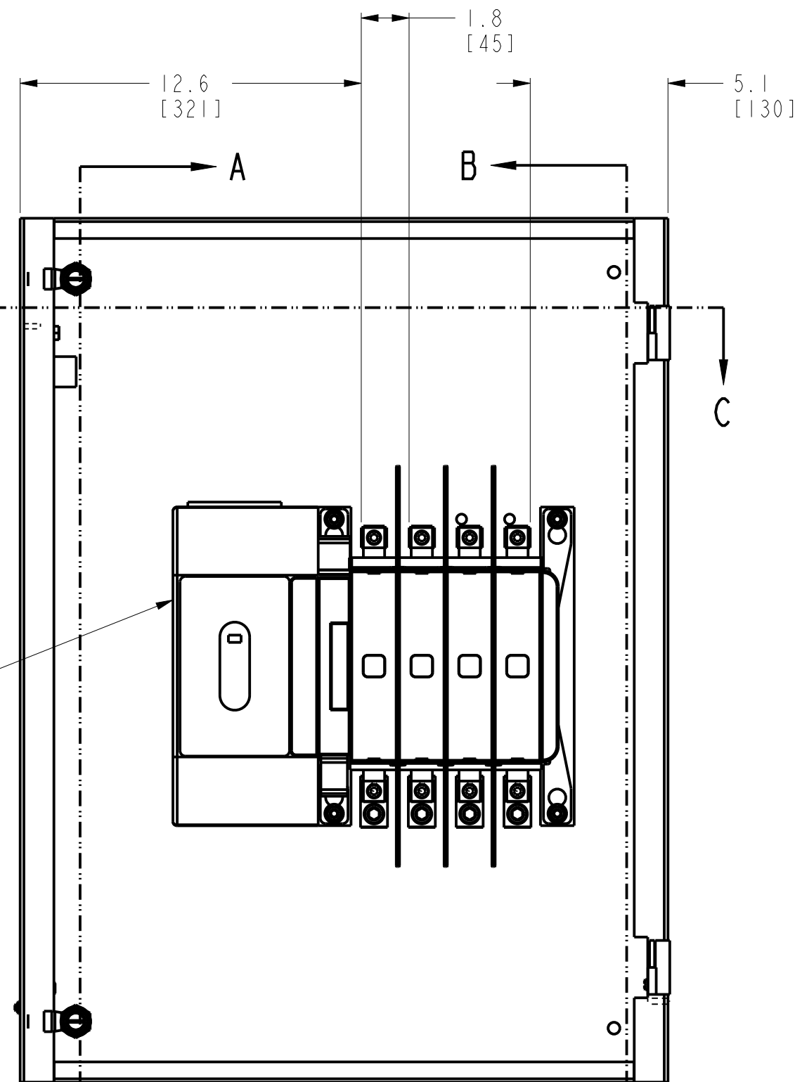
FRONT VIEW WITHOUT DOOR
