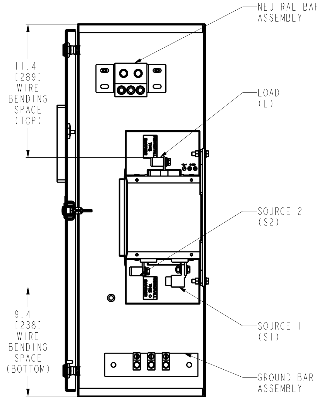
SECTION B-B RIGHT SIDE WITHOUT SIDE PANEL
