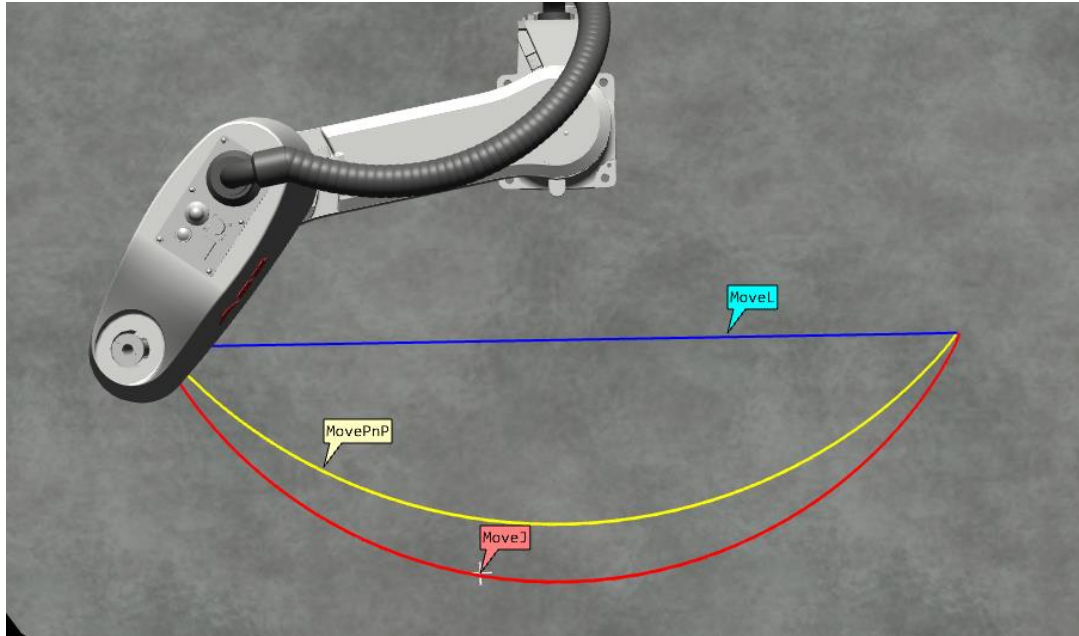
Figure 7. The picture shows an example of the MovePnP from the top view. The yellow path shows the trace of the MovePnP and the blue and red traces are examples of the corresponding motion programmed with MoveL and MoveJ, respectively.
