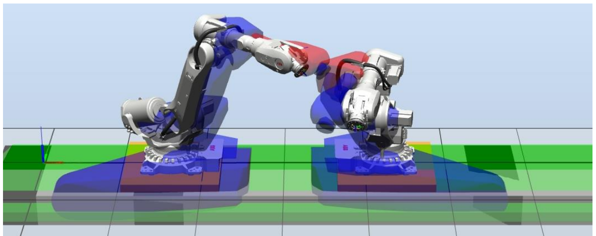
Figure 6. The same robots as in Figure 5 viewed in Online Monitor. It shows the collision predicted by the controller. The controller will stop the robot to prevent the collision from occurring.
