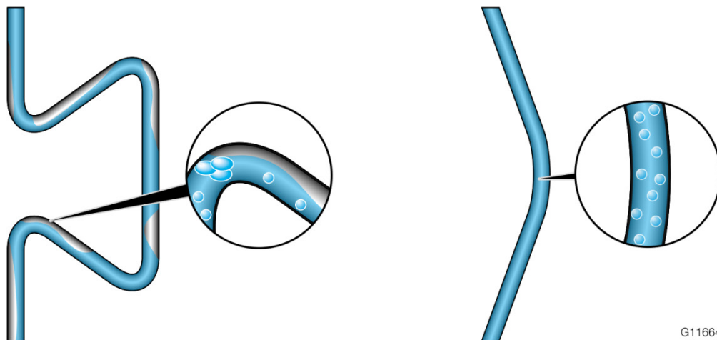
Fig. 2: Coriolis tube design largely determines the behavior of the meter in presence of gas phase
