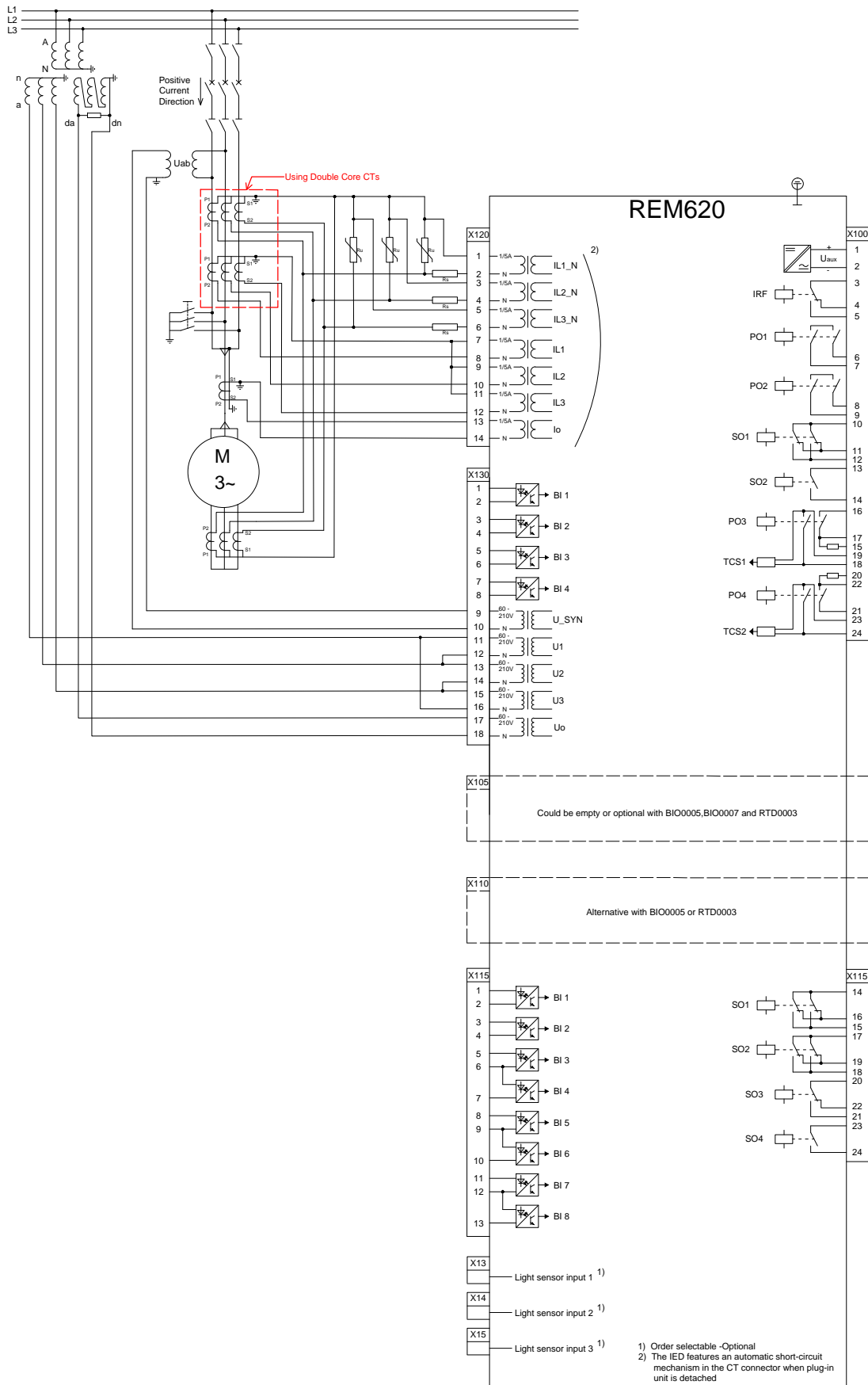
Figure: REM620 ME201 Connection diagram for standard modules ( For High-impedance based differential protection)
