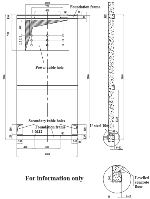
UniGear ZS3.2 Guideline structural data for foundation frame on concrete floor
