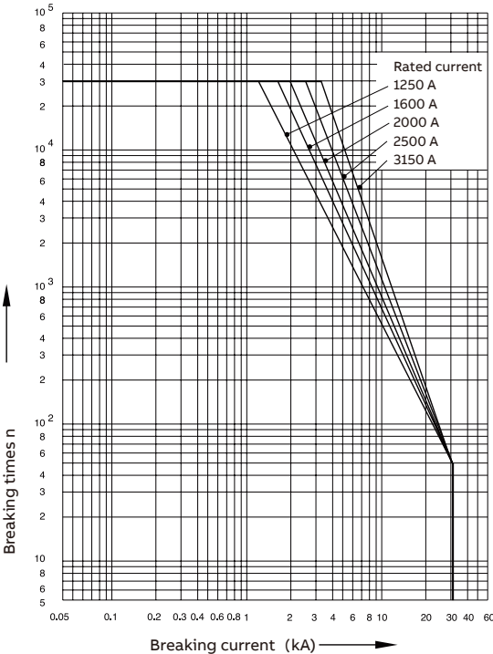
b) 40.5 kV, 1250...3150 A, 31.5 kA
