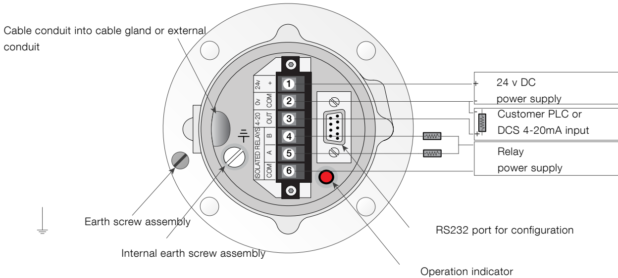
Typical LM80 24V DC electrical installation
