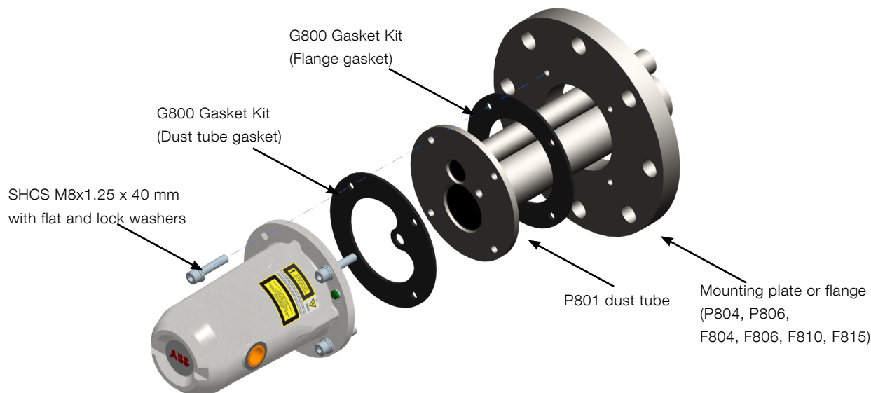
Typical LM80 installation with dust tube (P801) and flange
