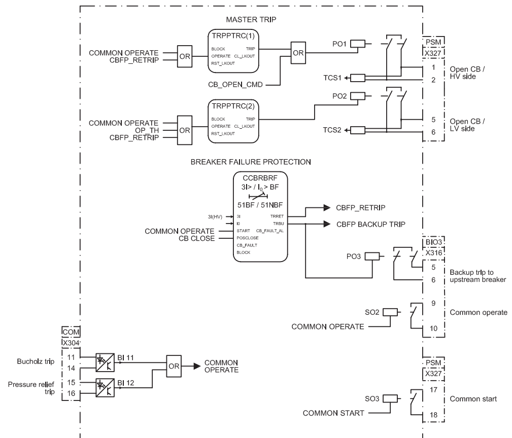
Figure 14: Tripping logic
