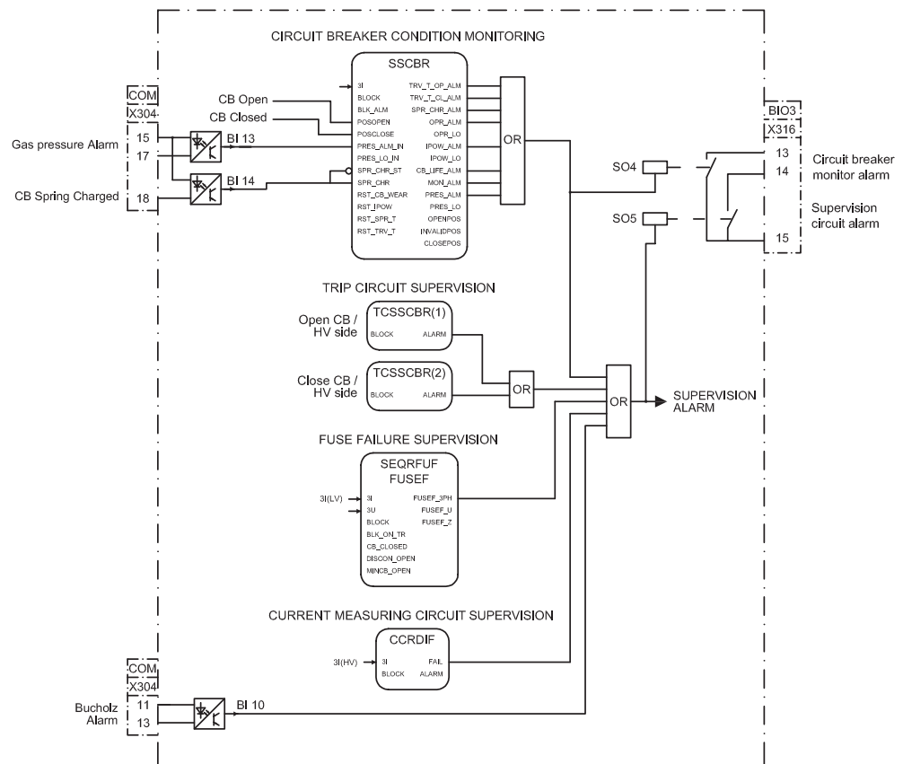
Figure 15: Circuit-breaker condition monitoring
