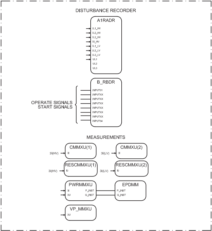
Figure 16: Measurement and analog recording
