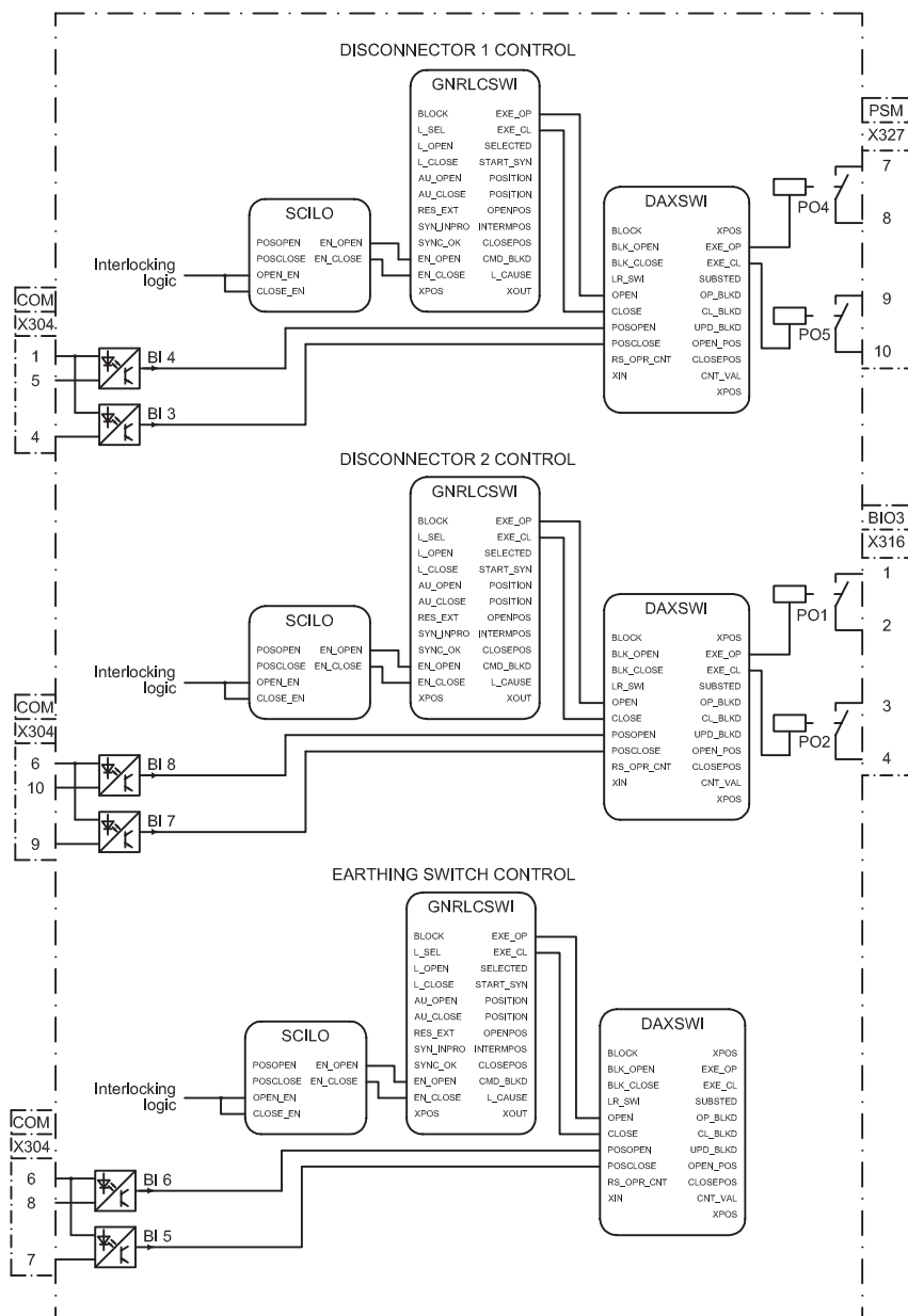
Figure 19: Disconnecter control
