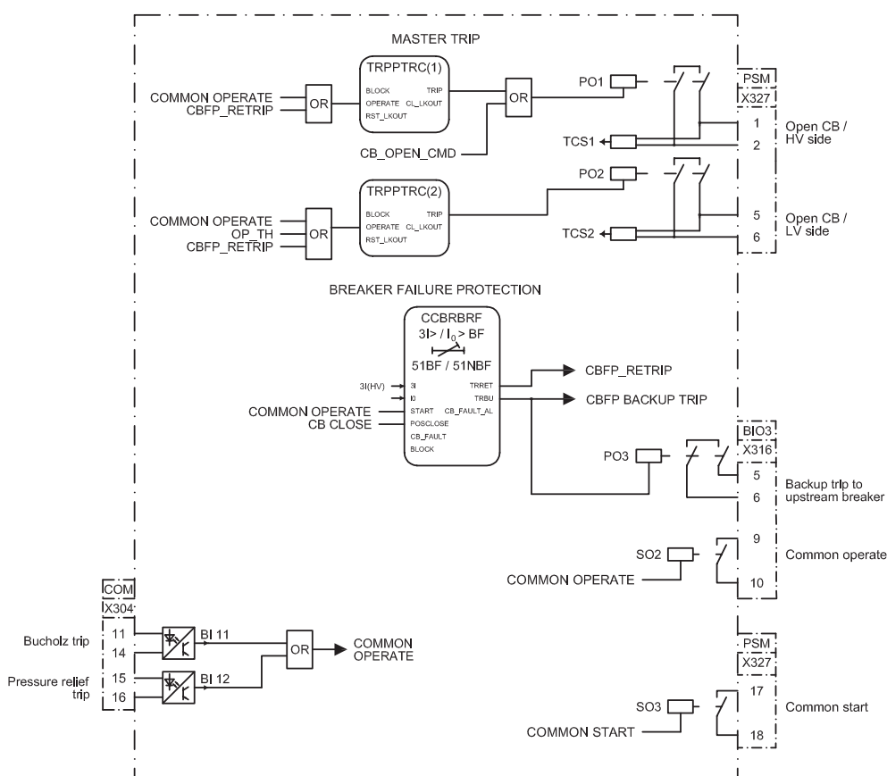
Figure 24: Tripping logic
