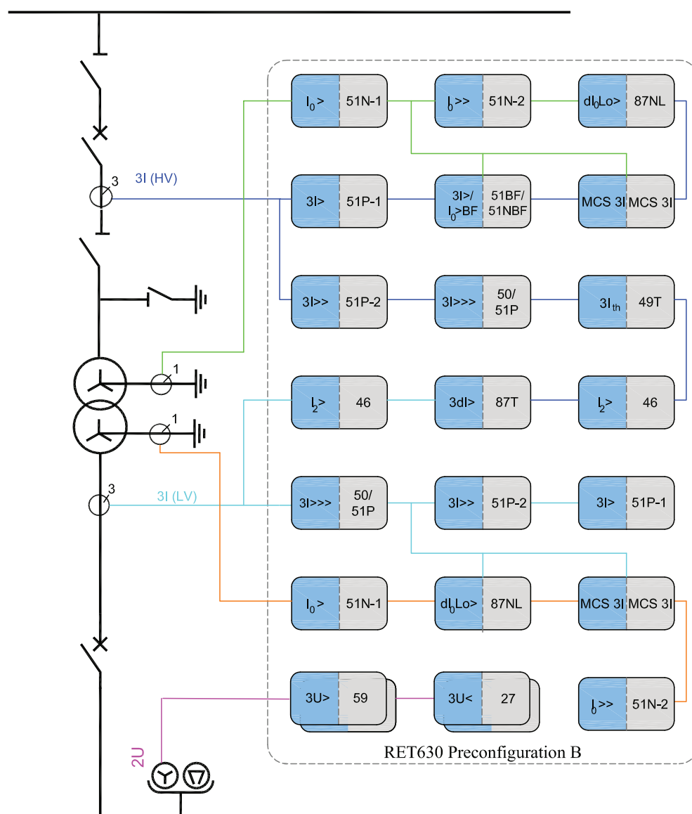
Figure 17: Single-line diagram for preconfiguration B for two-winding HV/MV transformer, including numerical REF protection
