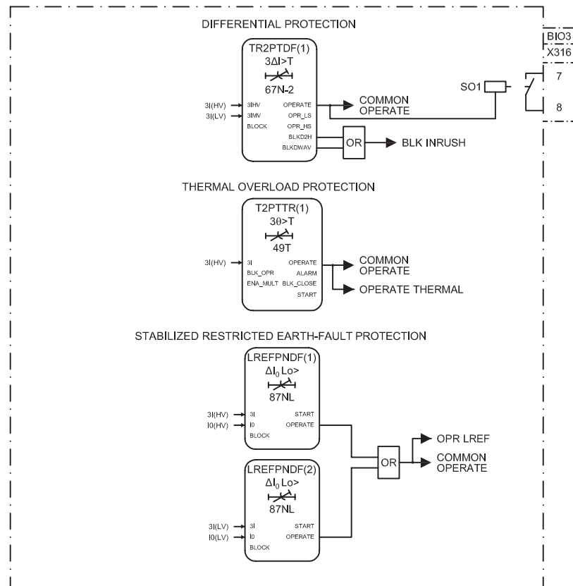
Figure 22: Thermal overload protection
