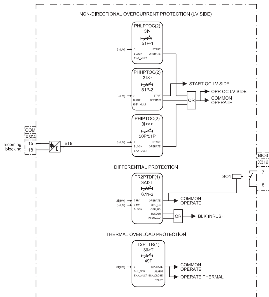
Figure 12: Thermal overload protection
