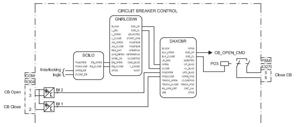
Figure 9: Circuit breaker control
