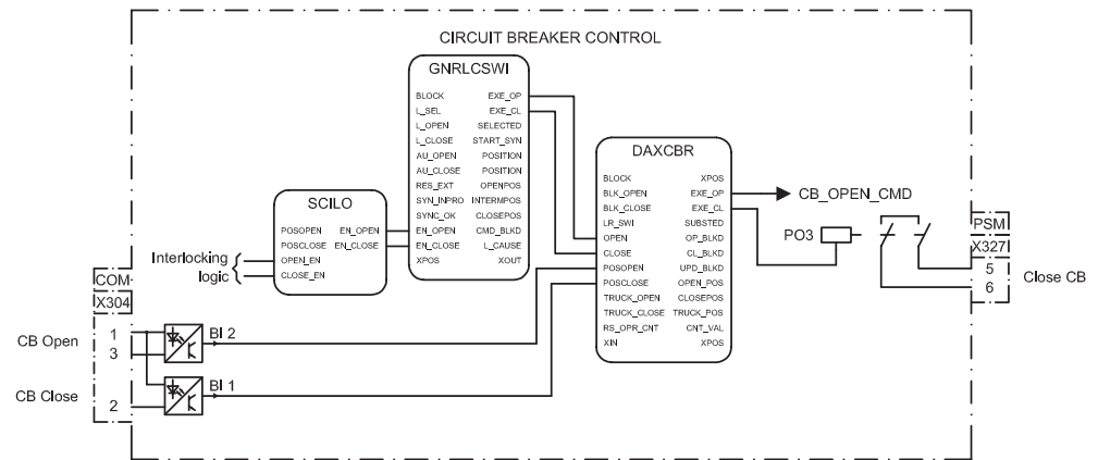
Figure 18: Circuit breaker control
