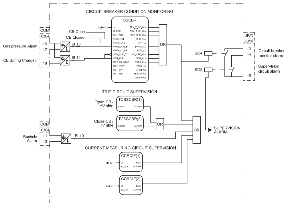
Figure 25: Circuit-breaker condition monitoring
