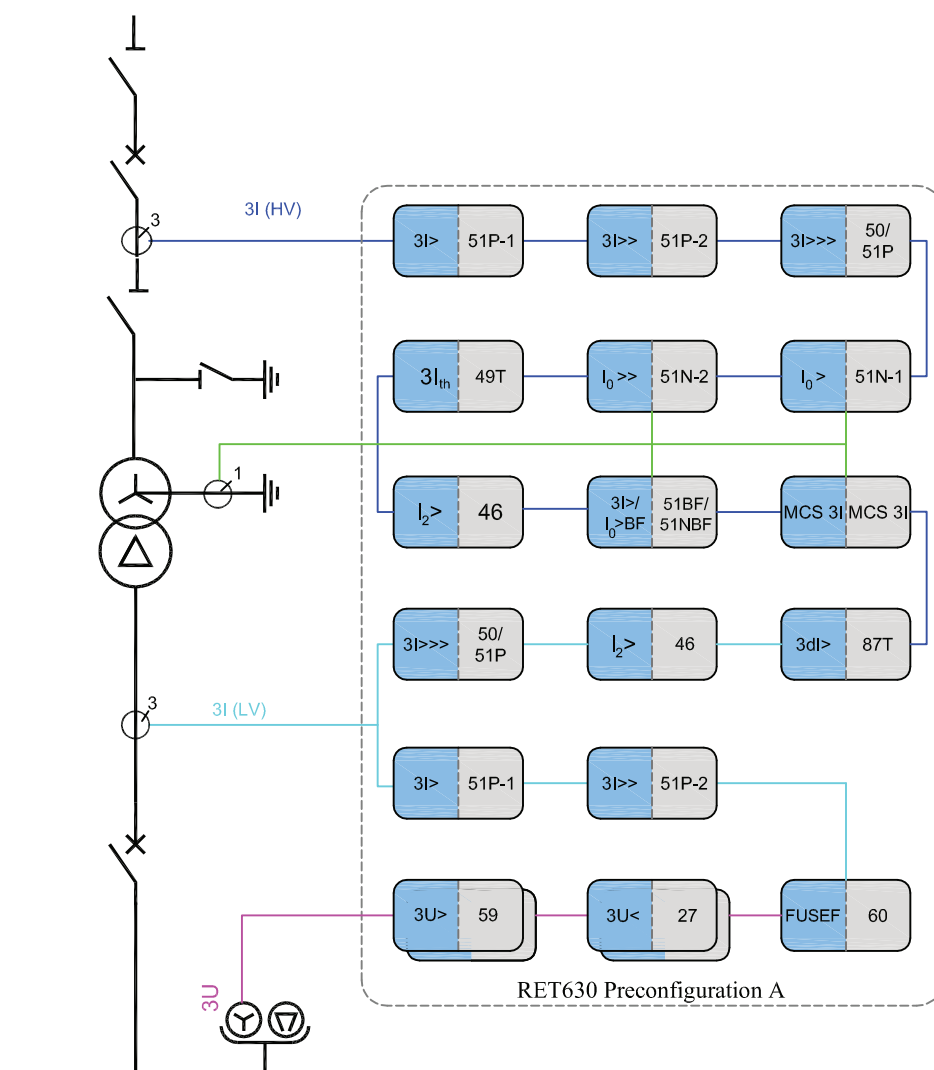
Figure 8: Single-line diagram for preconfiguration A for two-winding HV/MV transformer
