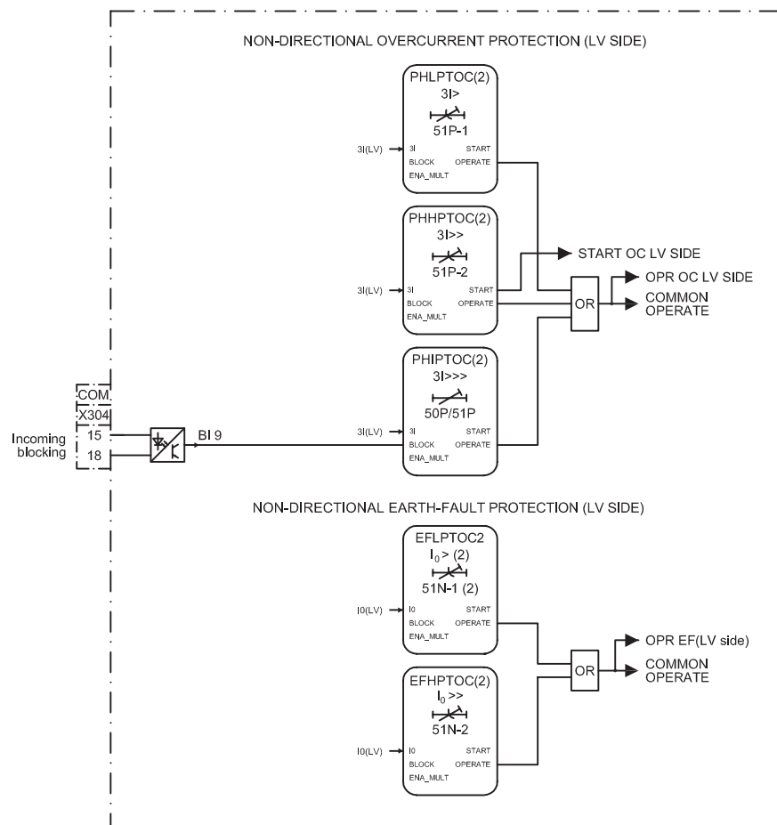
Figure 21: Non-directional earth-fault protection
