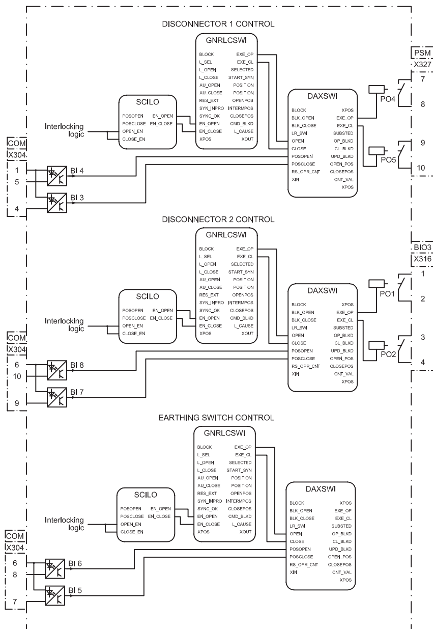
Figure 10: Disconnector control
