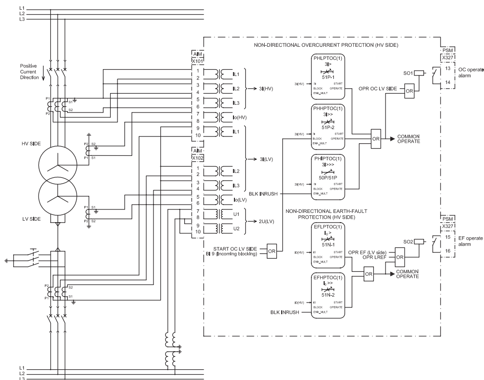
Figure 20: Non-directional overcurrent protection
