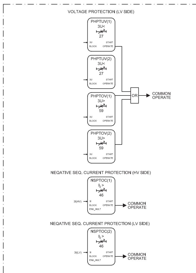
Figure 23: Three-phase undervoltage protection
