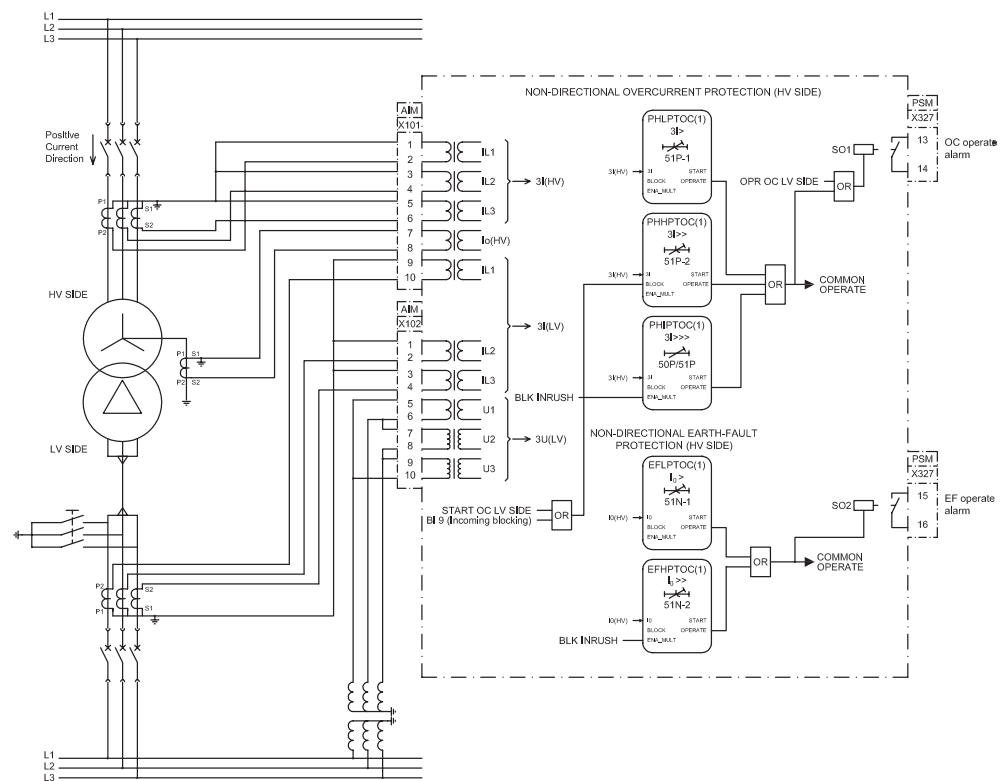
Figure 11: Non-directional overcurrent protection
