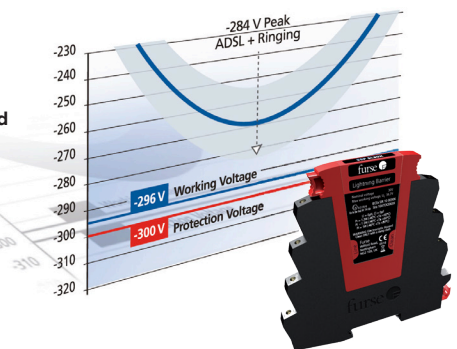
Graph 2: Maximum System Voltage with superimposed ADSL Signal
