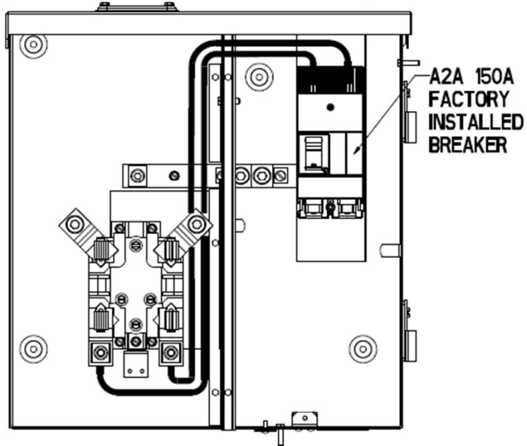
FRONT VIEW (DOORS OPEN CONDITION)
