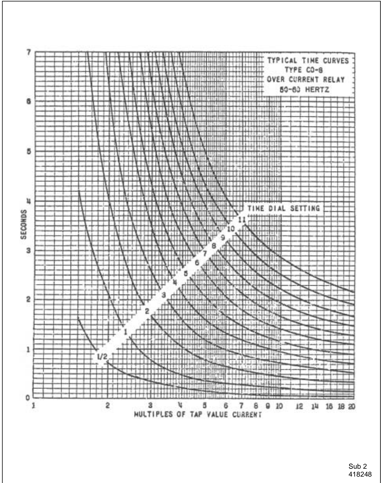
Figure 19. Typical Time Curve of the Time Overcurrent Unit of the Inverse (8) Relay
