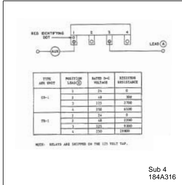
Figure 14. Selection of Proper Voltage Tap for Auxiliary Switch (CS-1) Operation
