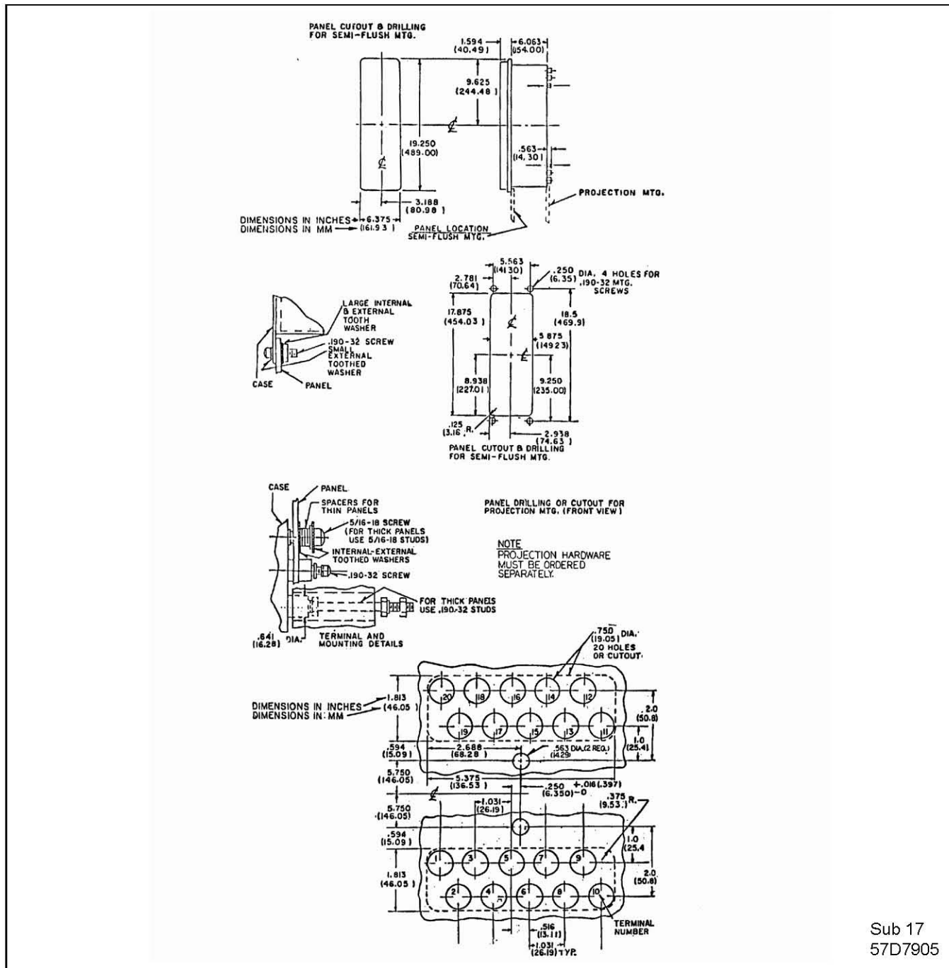
Figure 22. Outline and Drilling Plan for the Type IRQ Relay in the FT-42 Case
