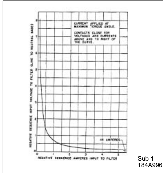
Figure 5 .Sensitivity Curve of the Directional Unit (D)
