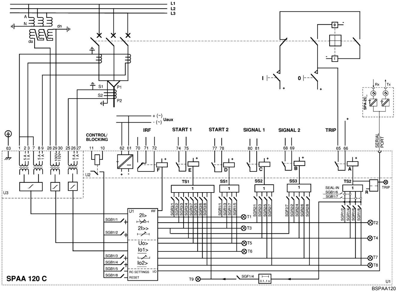
Fig. 10 Block diagram and sample connection diagram
