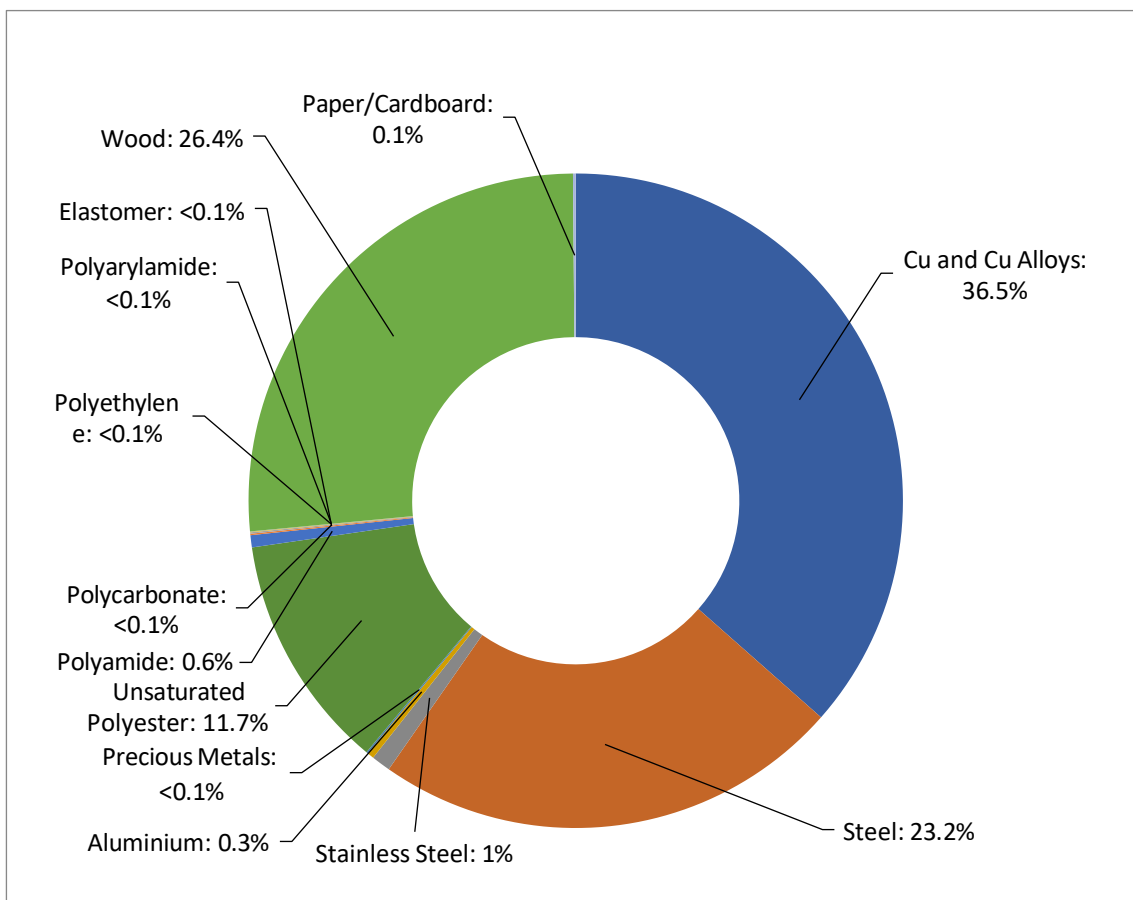
Figure 1: Material composition of HBRF Megamax F2-E2_2_W_HR_3P KIT IEC to E2.2 IEC
