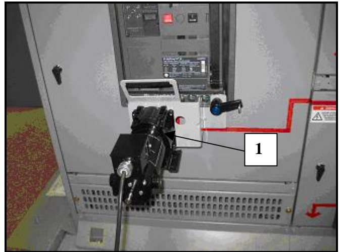
Fig. 4 Remote Racking Operator drive train
