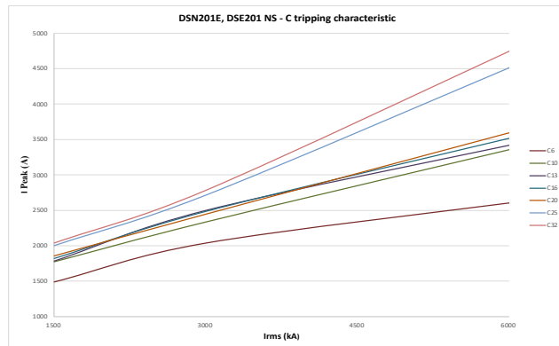
DSN201E, DSE201 NS - C tripping characteristic
