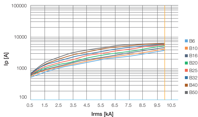
DSE201M, characteristic B
