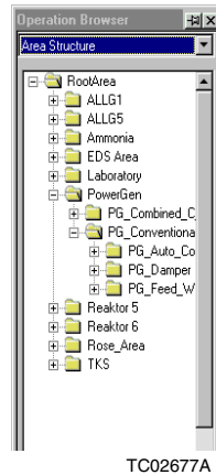
Figure 3. Object Browser
