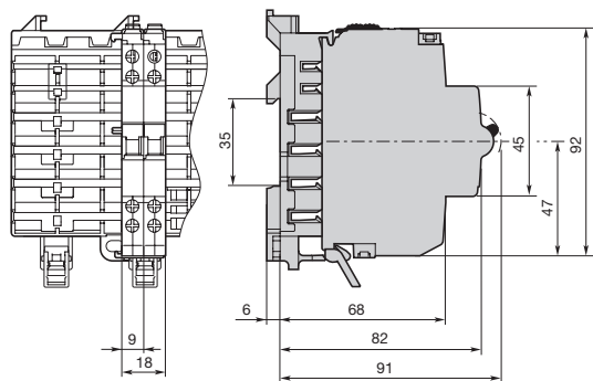
Auxiliary switch and signal contact
