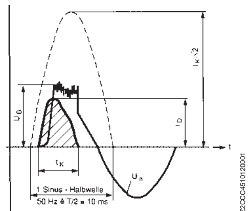
Oscillogram of a short circuit current interruption
