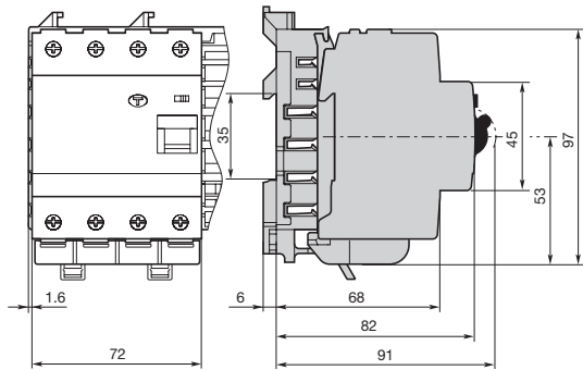
4-pole residual current operated circuit breaker, switch disconnecter and surge arrester
