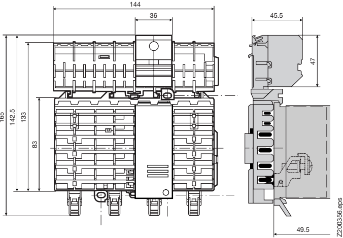
Incoming terminal component
