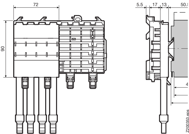
Universal adapter 100 A
