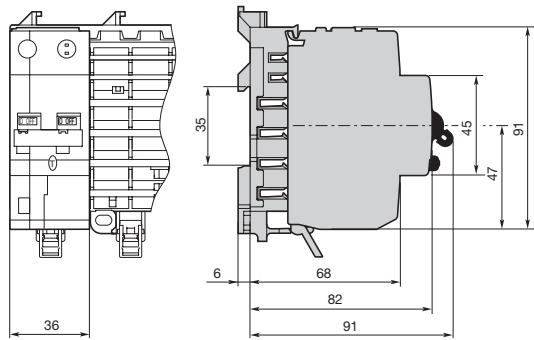
2-pole residual current operated circuit breaker
