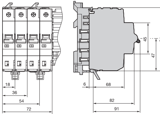
1-, 2-, 3- and 4-pole miniature circuit breakers
