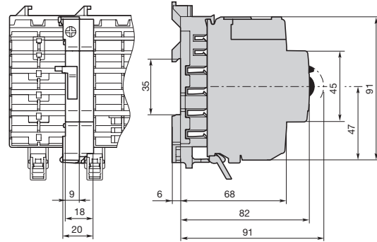
Neutral disconnecter
