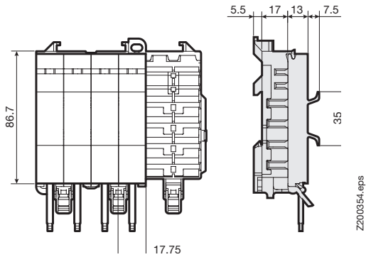
32A and 63A universal adapter
