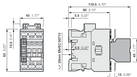
AFC26..K, AFC30..K, AFC38..K + CA4..K 1-pole auxiliary contact block
