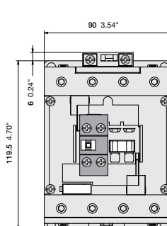
AFC80 + CA4 2-pole auxiliary contact
