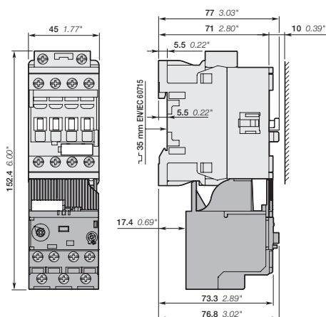
AFC09, AFC12, AFC16 3-pole contactors
