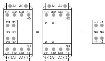
Combination 21 = AFC09 ... AFC16-30-10 + CA4-11
