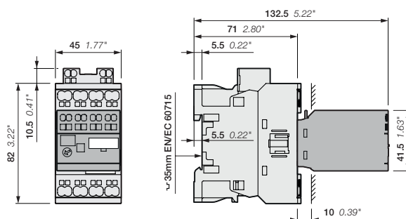
NFC22EK, NFC31EK, NFC40EK + TEF4S electronic timer
