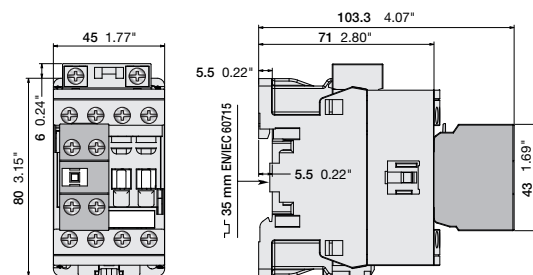
AFC09, AFC12, AFC16 + CA4 2-pole auxiliary contact
