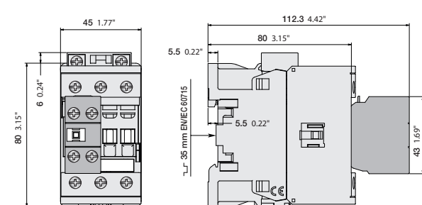
AFC26, AFC30, AFC38 + CA4 2-pole auxiliary contact
