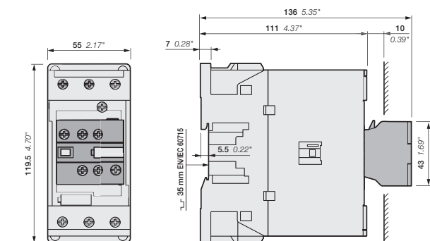
AFC40, AFC52, AFC65 + CAT4 2-pole auxiliary contact and coil terminal block
