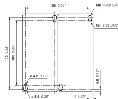
AFC40, AFC52, AFC65 + VM96-4 mechanical interlock set
