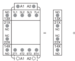
Combination 11 = CAL4-11 + AFC09 ... AFC80-40-00
