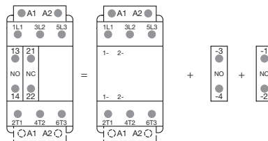
Combination 11 = AFC26 ... AFC96-30-00 + CA4-10 + CA4-01 (1)
