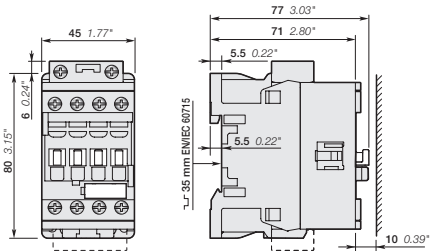
NFC22E, NFC31E, NFC40E Main dimensions mm, inches
