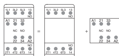
Combination 21 = AFC09 ... AFC16-30-10 + CAT4-11M
