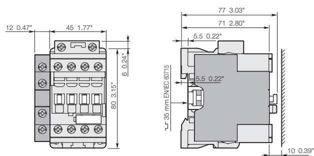
AFC09, AFC16 + CAL4-11 2-pole auxiliary contact block
