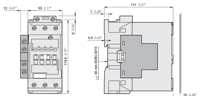
AFC40, AFC52, AFC65-30-00 + CAL4-11 2-pole auxiliary contact block AFC40, AFC52, AFC65-30-11
