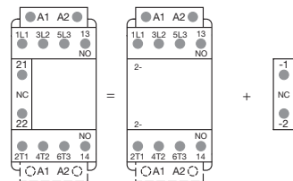
Combination 11 = AFC09 ... AFC16-30-10 + CA4-01 (1)
