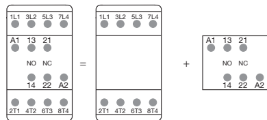
Combination 11 = AFC09 ... AFC80-40-00 + CAT4-11E
