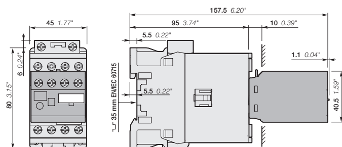
AFC26, AFC38 + TEF4 electronic timer
