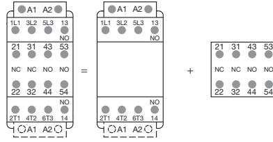
Combination 32 = AFC09 ... AFC16-30-10 + CA4-22M (1)
