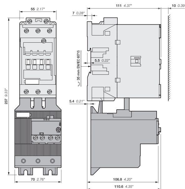
AFC40, AFC52, AFC65 + EF65 electronic overload relay
