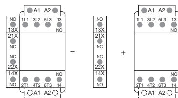
Combination 21 = CAL4-11 + AFC09 ... AFC16-30-10 (1)
