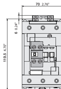
AFC80, AFC96 + CA4 2-pole auxiliary contact
