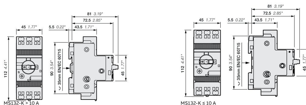
Main dimensions mm, inches
