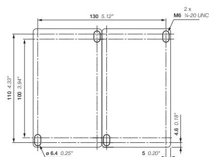
AFC40, AFC52 + VM96-4 mechanical interlock unit
