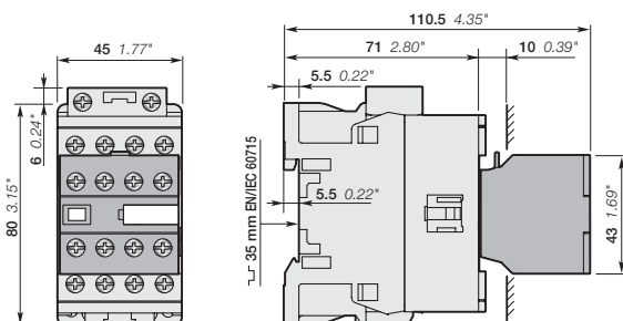
AFC09, AFC16 + CA4 4-pole auxiliary contact block
