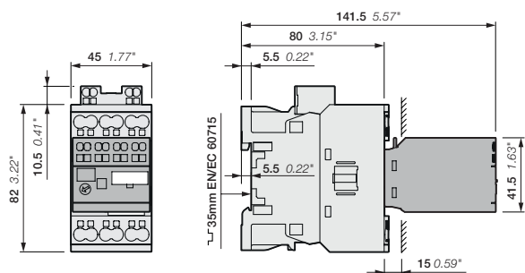
AFC26..K, AFC30..K, AFC38..K + TEF4S electronic timer
