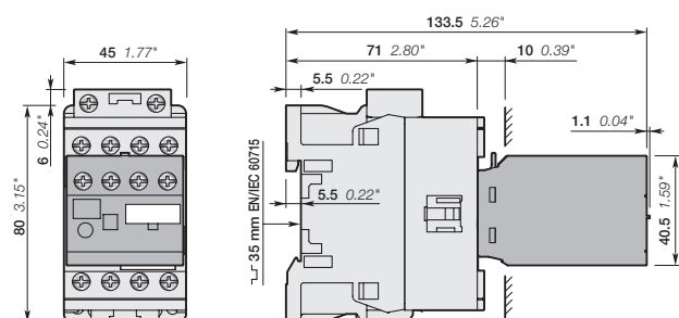
AFC09, AFC16 + TEF4 electronic timer
