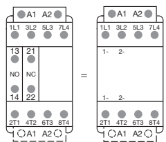
Combination 11 = AFC09 ... AFC80-40-00 + CA4-10 + CA4-01
