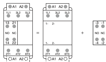
Combination 11 = AFC26 ... AFC96-30-00 + CA4-11
