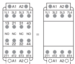
Combination 22 = AFC09 ... AFC80-40-00 + CA4-22E
