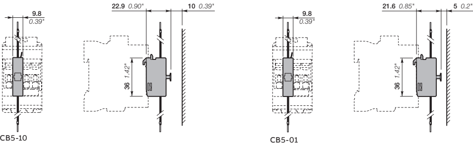
Main dimensions mm, inches
