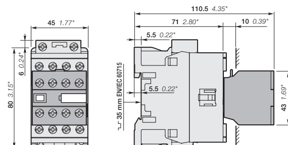
NFC22E, NFC31E, NFC40E + CA4 4-pole auxiliary contact block
