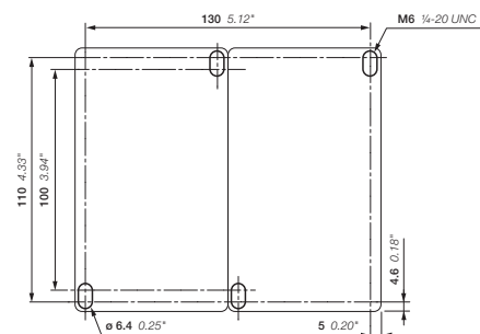
AFC80, AFC96 + VM96-4 mechanical interlock set
