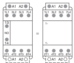
Combination 10 = AFC09 ... AFC80-40-00 + CA4-10
