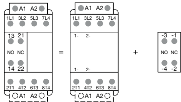
Combination 11 = AFC09...AFC80-40-00 + CA4-11
