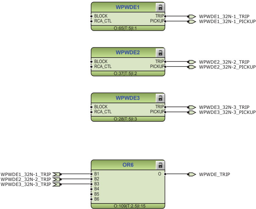
Figure 18: Wattmetric protection function
