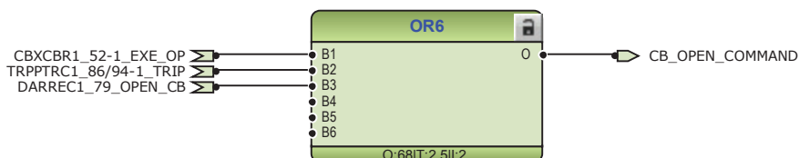
Figure 99: Circuit breaker control logic: Signals for the opening coil of circuit breaker 1
