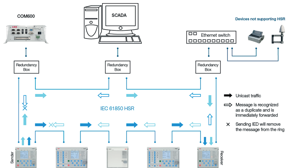
Figure 8: HSR solution
