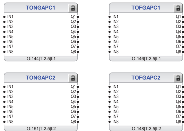
Figure 117: Programmable timers
