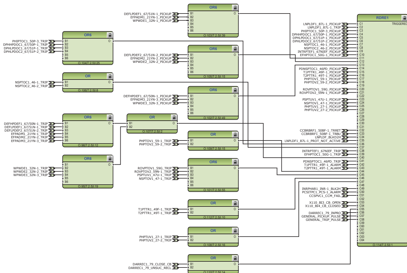
Figure 89: Disturbance recorder
