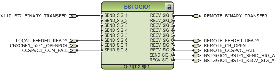
Figure 41: Binary signal transfer function
