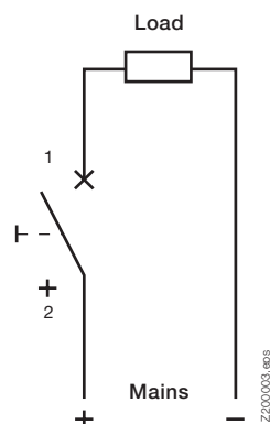
Connection diagram, single-pole (max. 220 V=) S401M-UCZ
