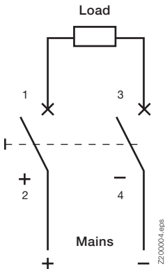
Connection diagram, two-pole (max. 440 V=) S402M-UCC
