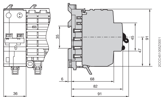
2-pole residual current operated circuit breaker F402
