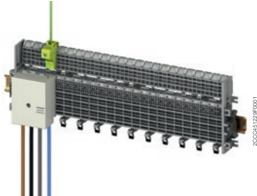
Power supply left or right, maximum 100 A. 125 A (max. 35 °C Ambient air temperature for 125 A continuously)
