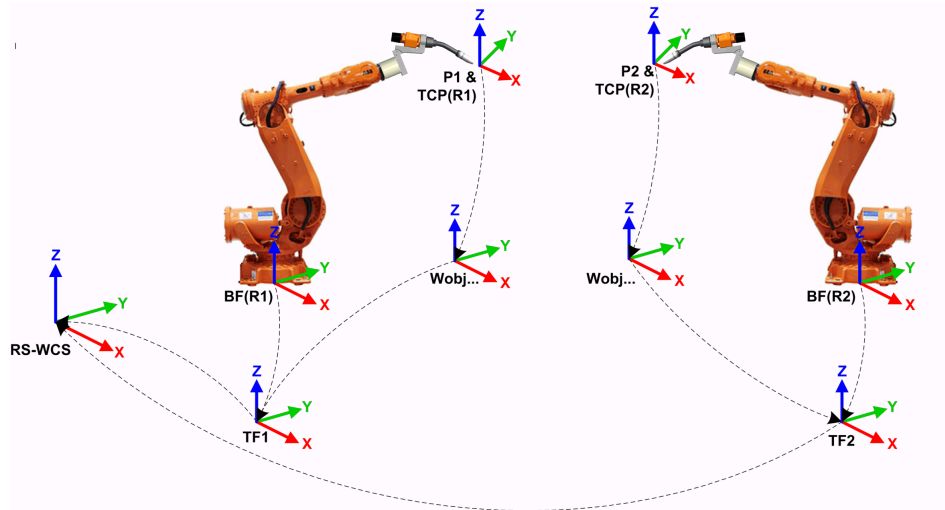
en1000001442_Station_with_Multiple_Robot_systems
