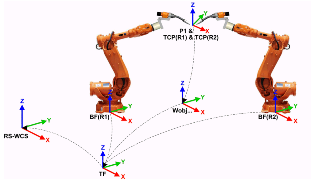
en1000001305_Coordinated_MultiMove
