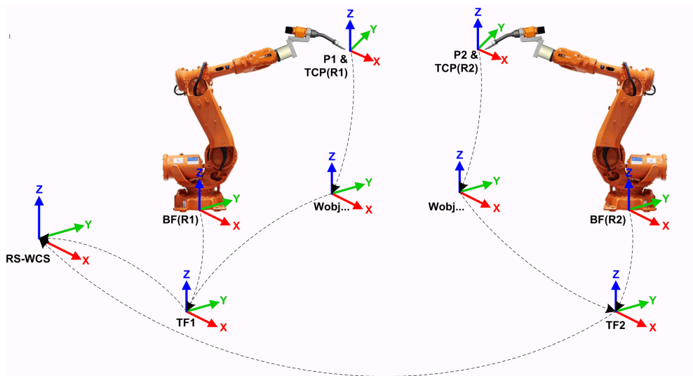
en1000001308_Independent_MultiMove
