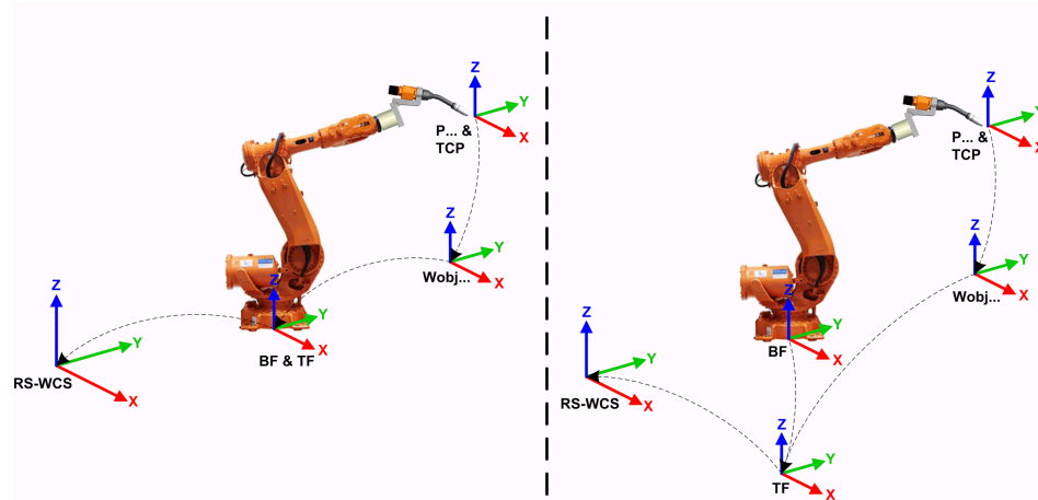
en1000001303_Taskframe_in_Same_and_Different_Positions
