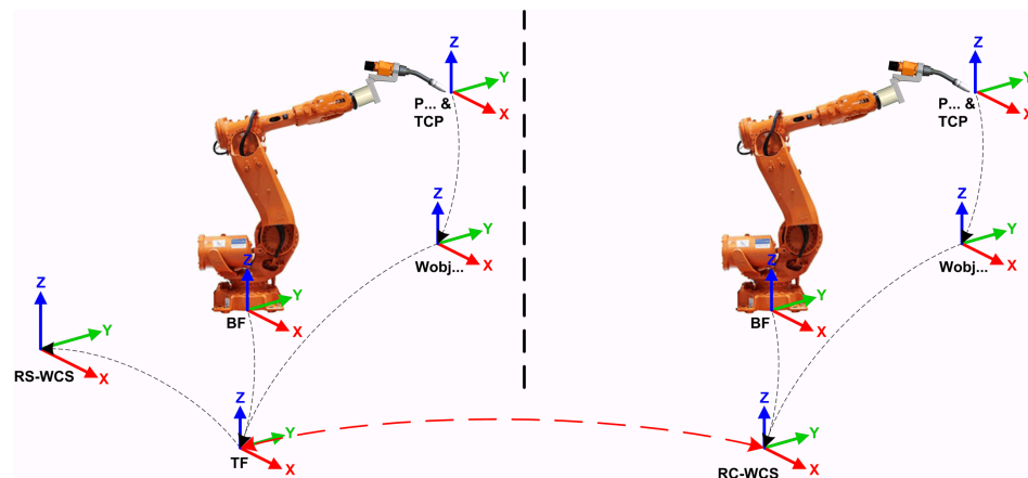
en1000001304_Taskframe_mapped_to_RC_Coordinate_System_in_Real_world
