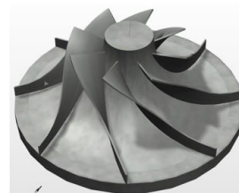
Defeated ~1 MB
