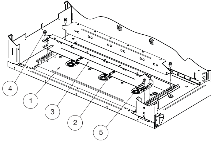
Figure 91. Medium voltage cable cover
