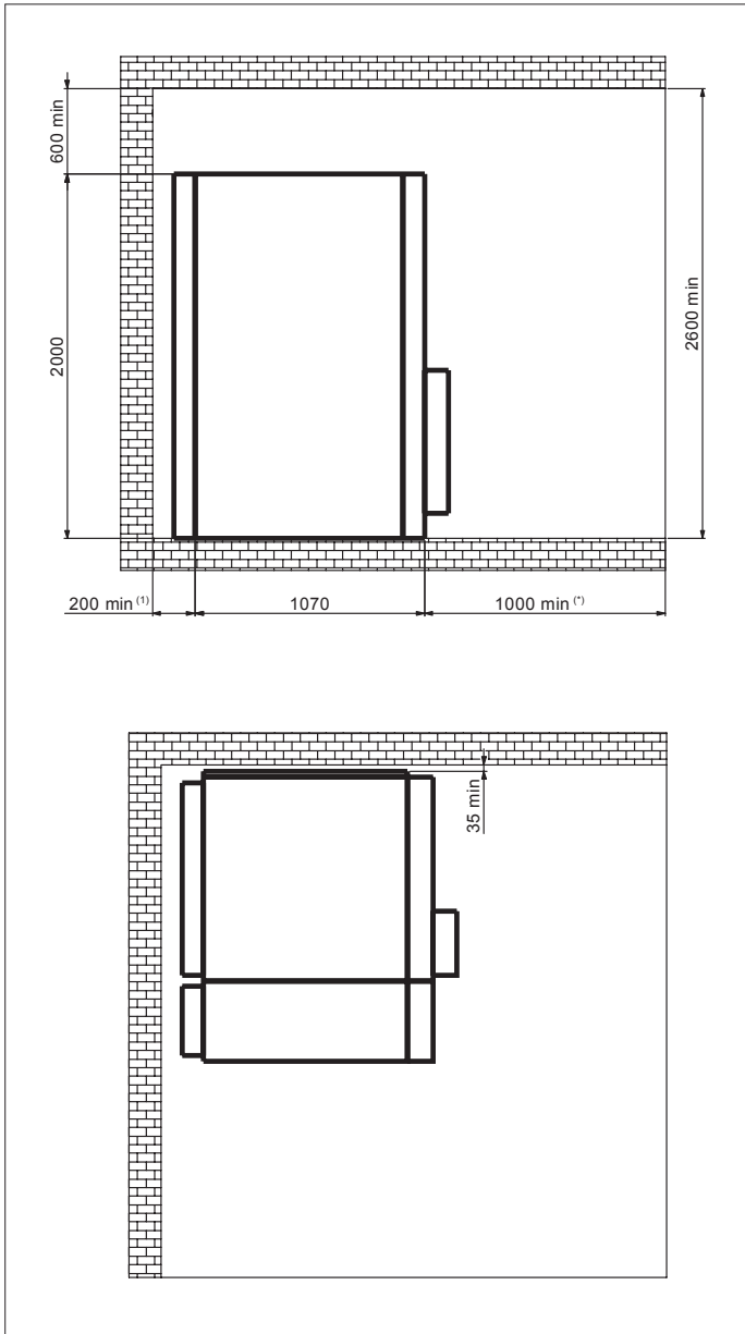
Figure 29. Minimum distances from the walls of the installation room, solution IAC A-FLR 21 kA 1s with filters installed on each unit
