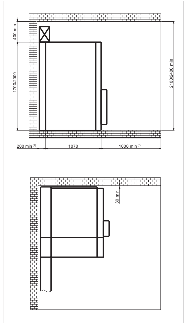
Figure 30. Minimum distances from the walls of the installation room, solution IAC A-FLR 21/25 (2) kA 1s with gas exhaust ducts
