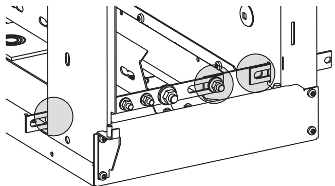
Figure 116. Busbar moved from the adjacent unit to the right
