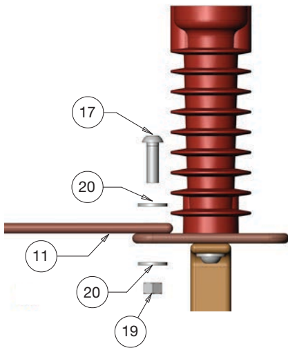
Figure 63. 630 A end unit
