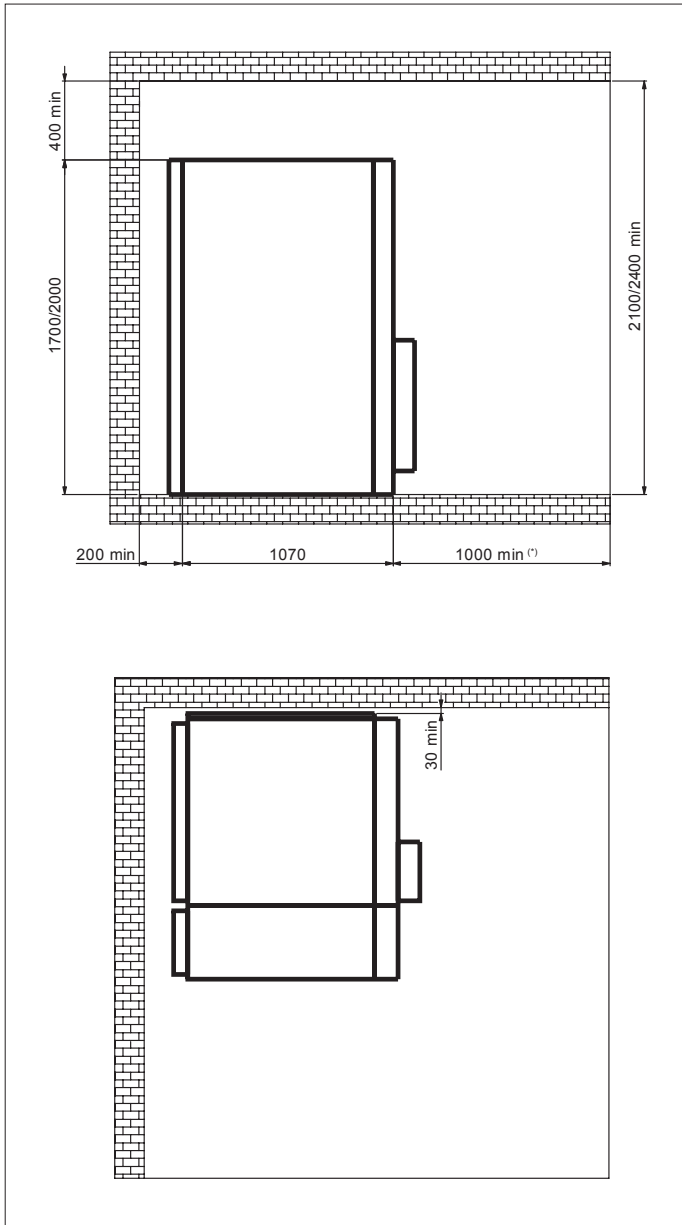
Figure 27. Minimum distances from the walls of the installation room, solution IAC A-FL 12.5 kA 1s with filters installed on each individual unit
