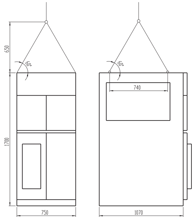
Figure 23. Dimensions and angles
