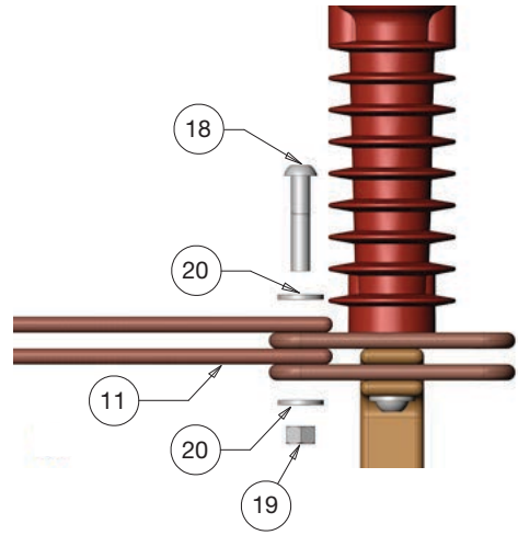
Figure 64. 1250 A end unit
