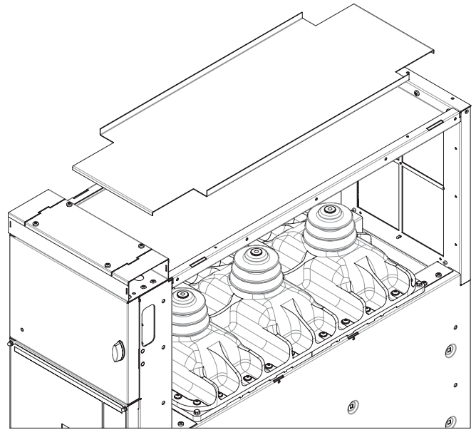
Figure 71. Installation of double roof plate
