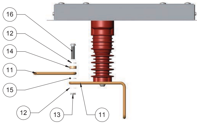
Figure 57. Busbar exit on the left
