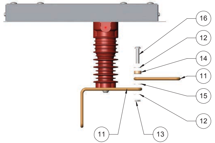
Figure 58. Busbar exit on the right
