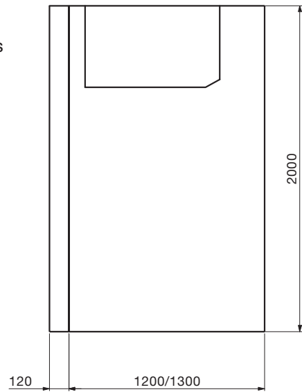
Figure 6. Side view for panels with withdrawable circuit-breakers, IAC A-FLR 25 kA, 1 sec up to 17.5 kV and IAC A-FLR 16 kA, 1s at 24 kV with filters
