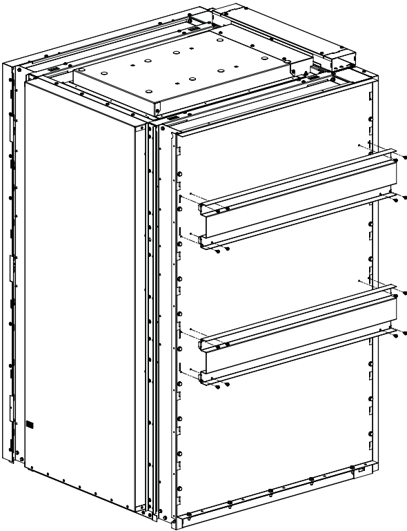
Figure 102. RLC transversal part
