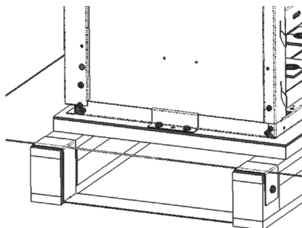
Figure 11. Fixing plates outside the 375-500 mm unit
