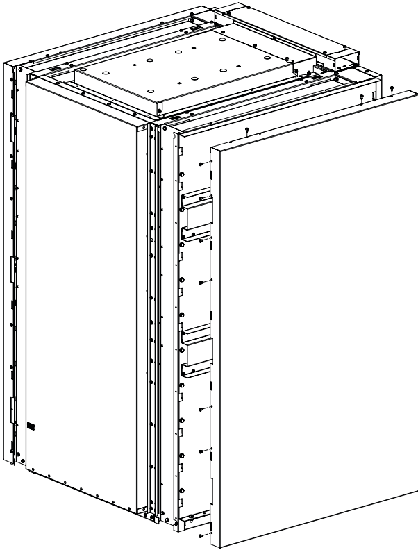
Figure 101. RLC cover
