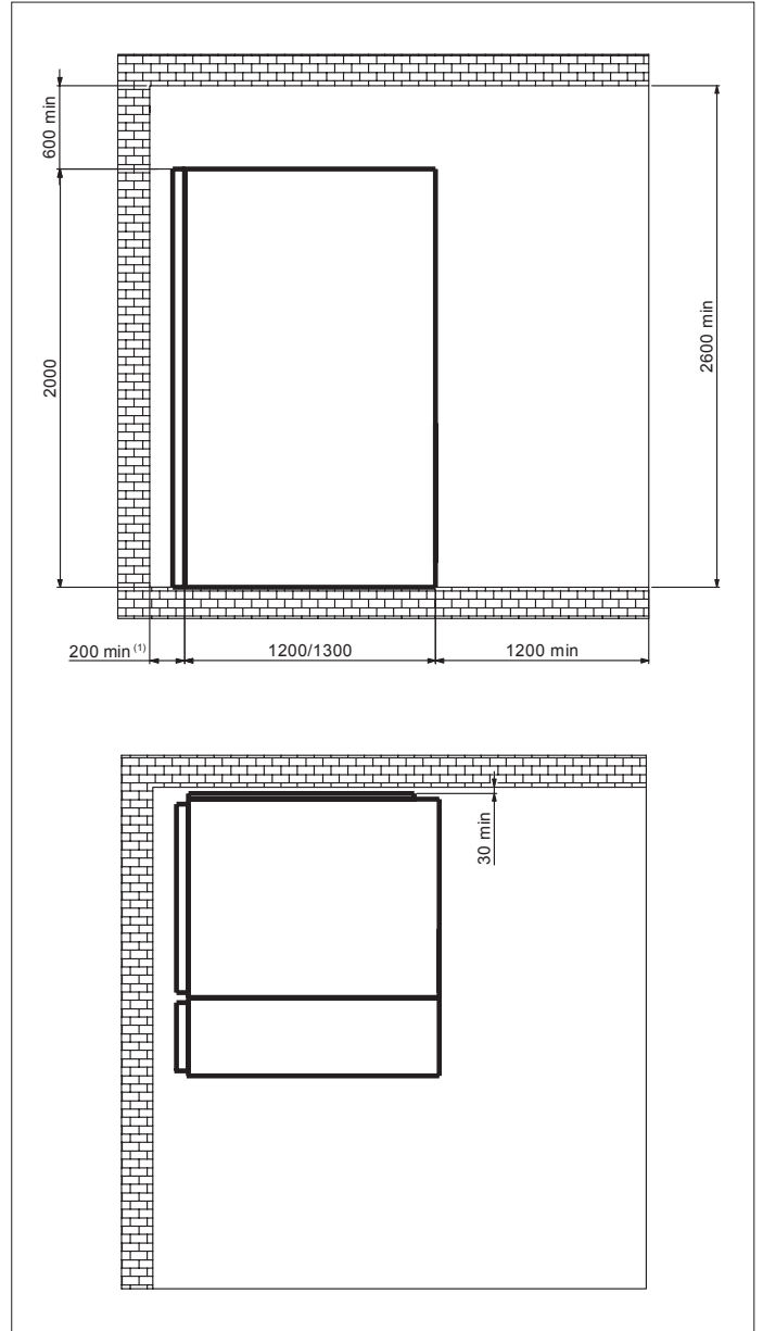
Figure 34. Minimum distances from walls of installation room, solution IAC A-FL 12.5 kA 1s with filters installed on each individual unit
