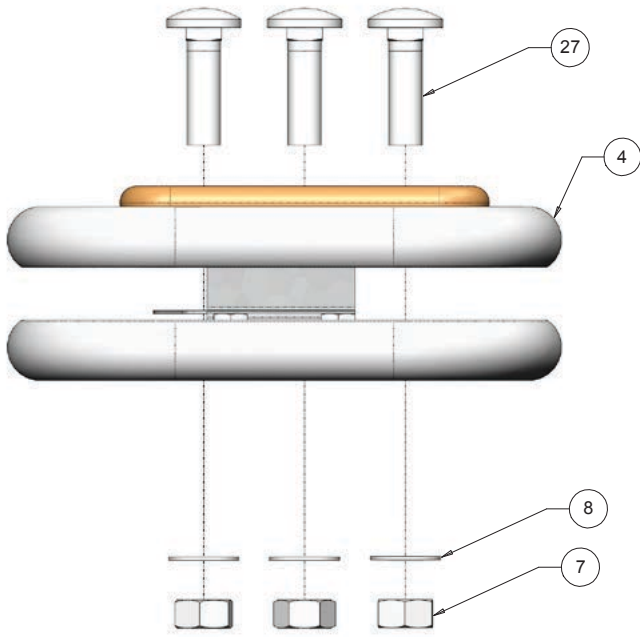
Figure 69. Busbar junction kit - 24 kV, 630 A
