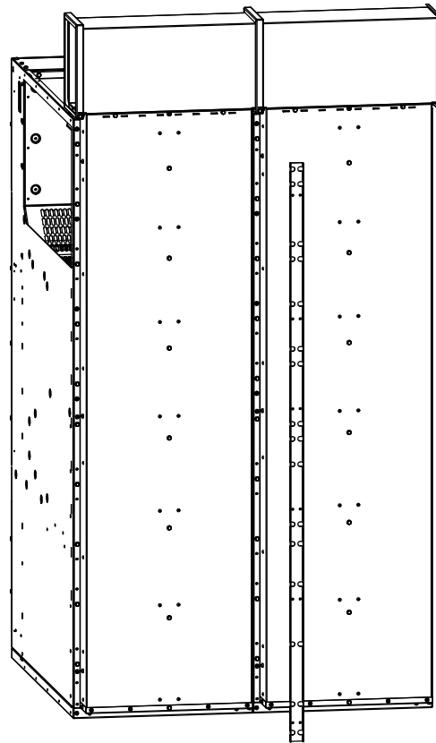
Figure 49. Screw positions for WBC – WBS units
