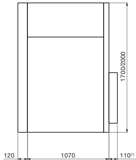
Figure 10. Side view of IAC AFLR 21kA x 1s - Downward
