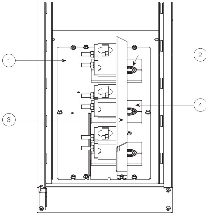
Figure 90. Parts
