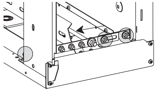
Figure 115. Busbar moved towards the adjacent unit on the left
