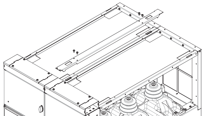
Figure 72. Outline of roof joining
