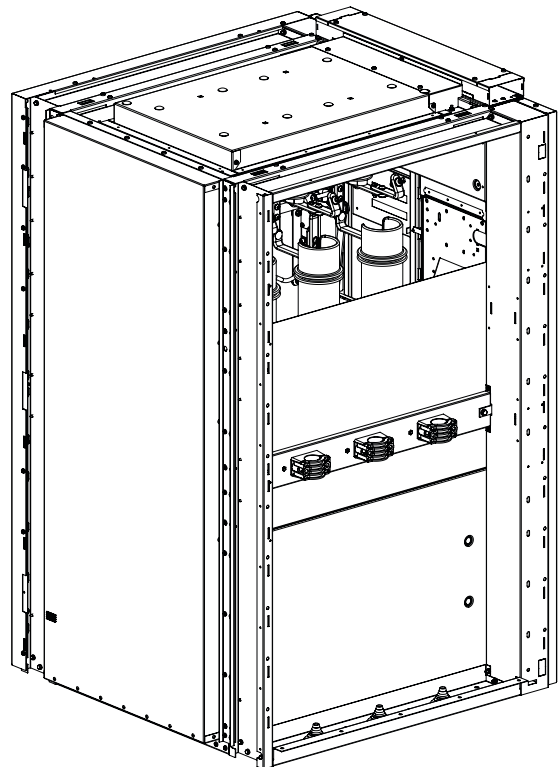
Figure 104. RLC unit cable locking parts
