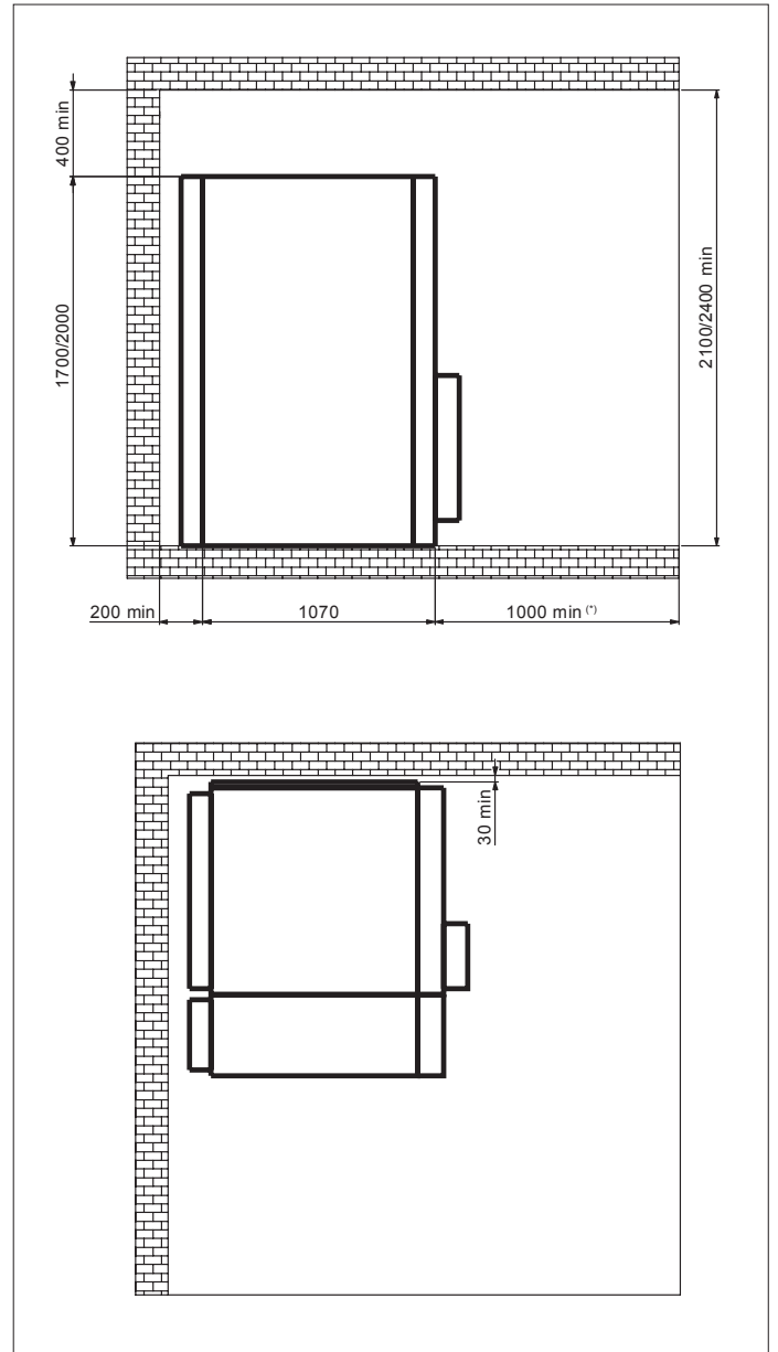
Figure 28. Minimum distances from the walls of the installation room, solution IAC A-FLR 16 kA 1s with filters installed on each unit
