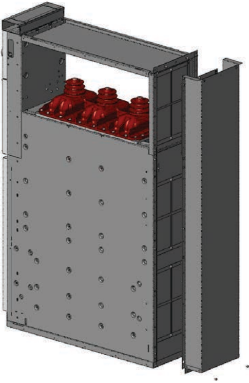
Figure 73. Installation of the vertical gas vent duct
