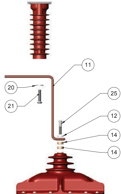
Figure 66. 12-17.5 kV, 630 A end unit
