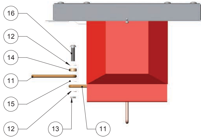
Figure 59. Busbar exit on the left
