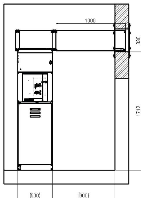
Figure 80. View from front
