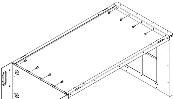
Figure 39. 500 mm wide units
