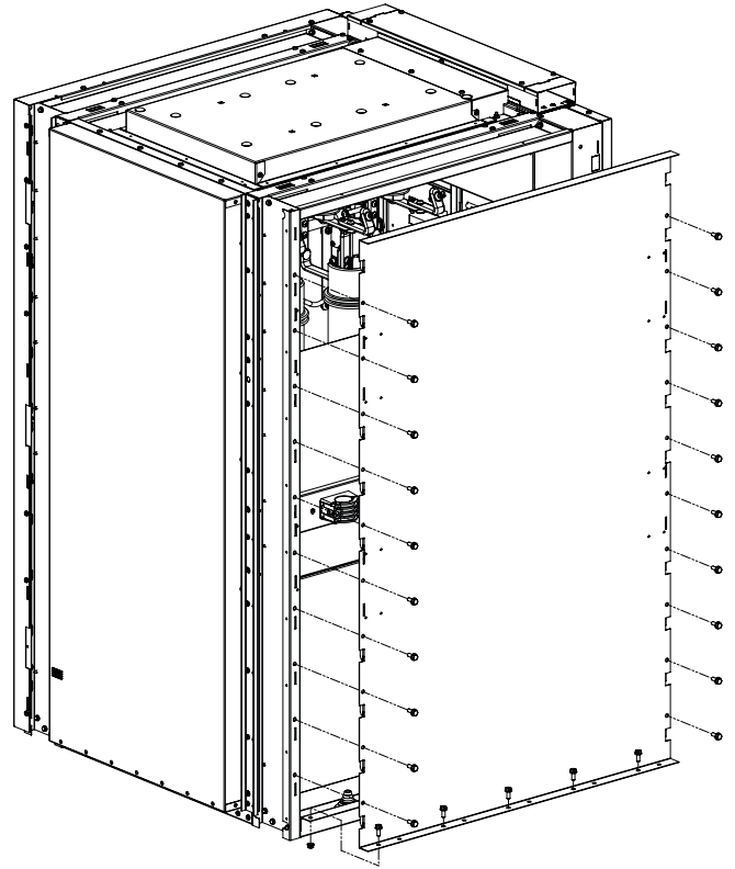
Figure 103. RLC internal cover
