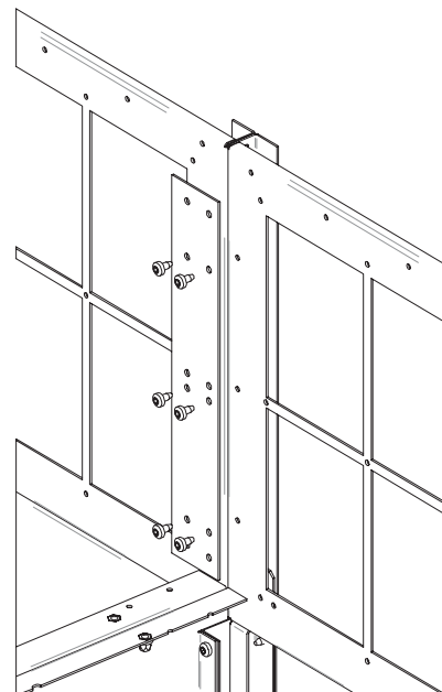
Figure 46. Plates installed
