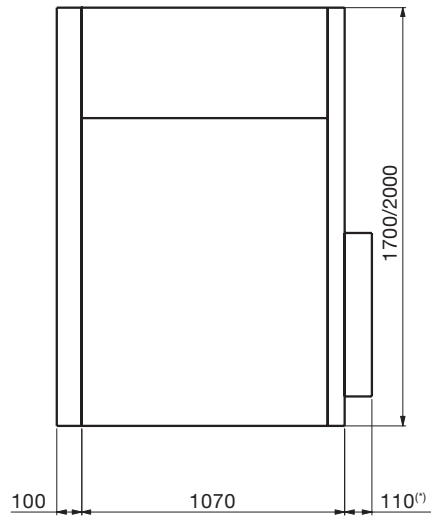
Figure 4. Side view IAC A-FLR 16 kA, with filters
