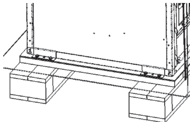
Figure 12. Fixing plates outside the 750 mm unit
