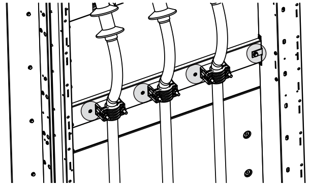
Figure 108. RLC unit earthing cable terminals
