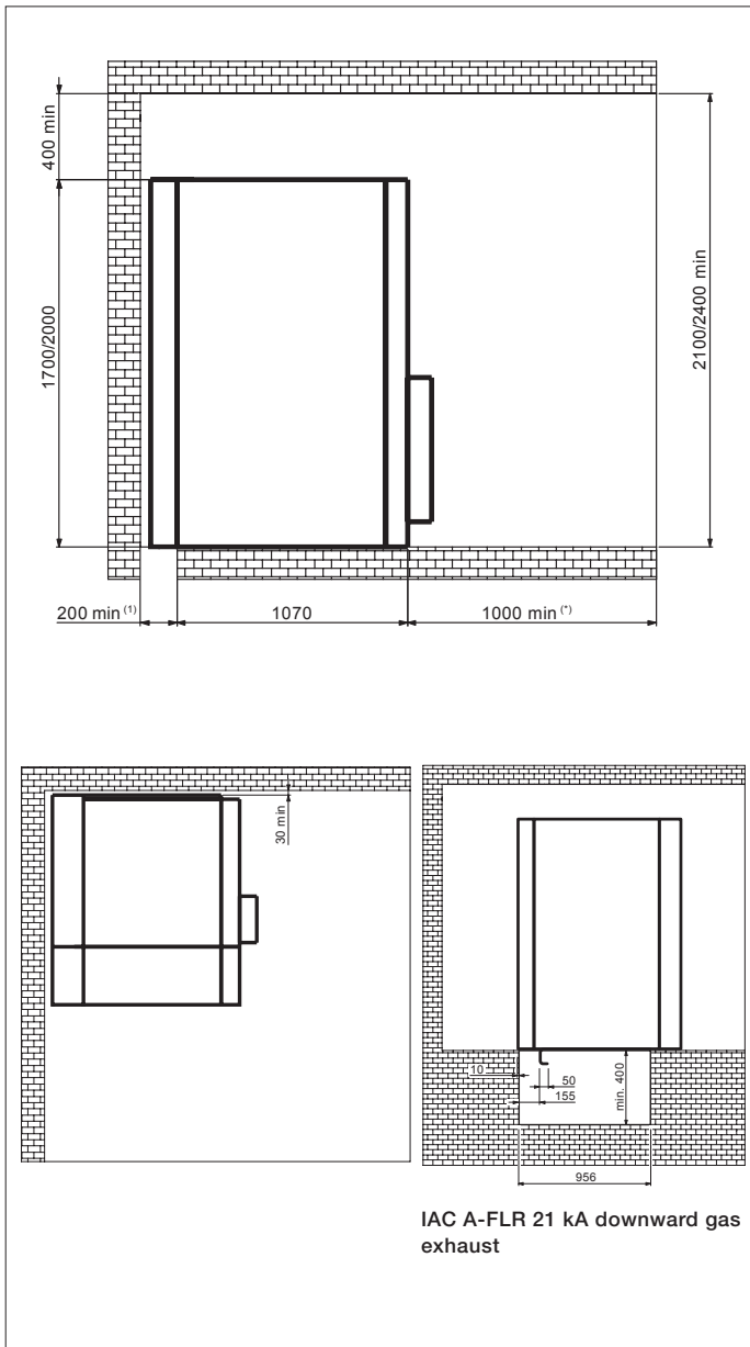
Figure 31. Minimum distances from walls of installation room, solution IAC A-FLR 21/25 (2) kA 1s with gas exhausted downwards
