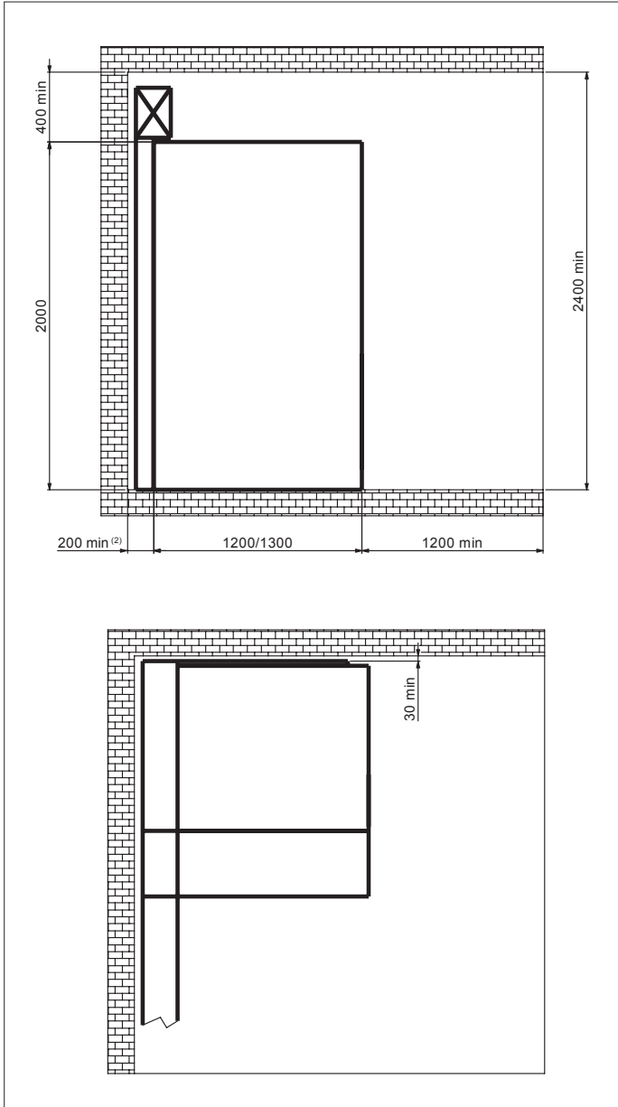
Figure 33. Minimum distances from the walls of the installation room, solution IAC A-FLR 25 kA, 1s @ 12-17.5 and 21 kA, 1s @ 24 kV with gas exhaust ducts
