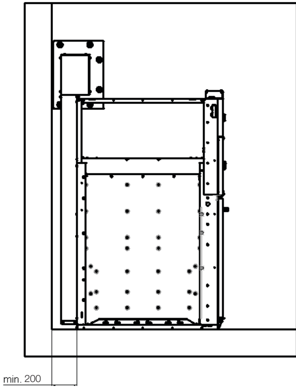
Figure 81. Side view
