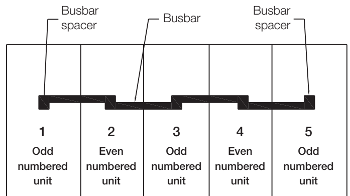
Figure 50. Main busbar connections
