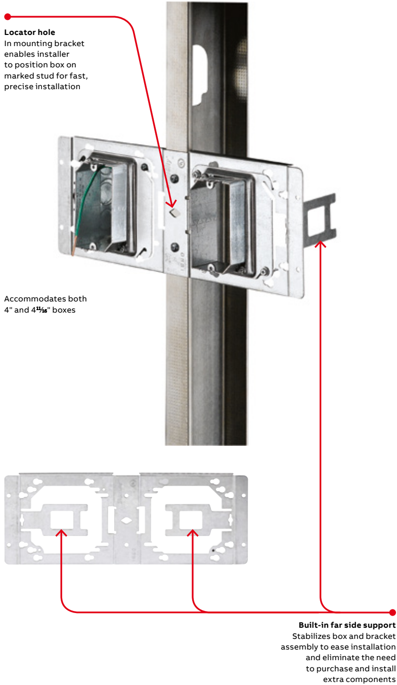
Power on both sides of the stud
