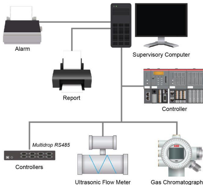
Figure 6.2 Example of a multi-drop system
