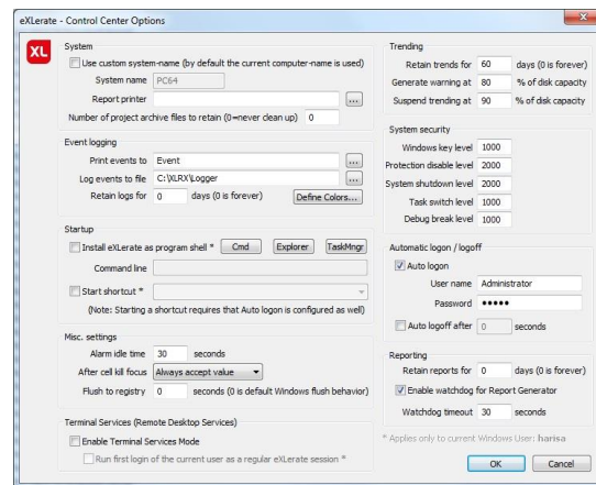
Figure 4.8 Control Center Options
