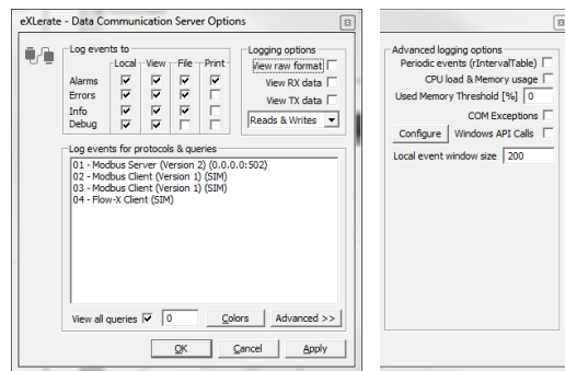
Figure 6.7 Communication server properties
