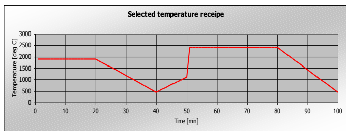
Figure 5.9 Temperature profile example
