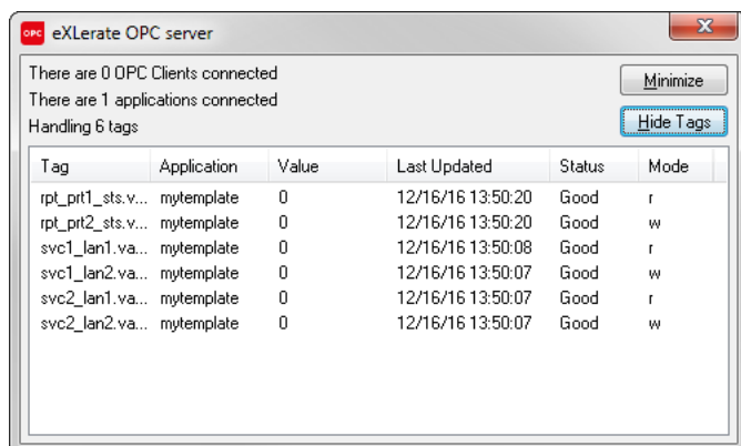
Figure 6.13 OPC monitor with tags hidden and shown
