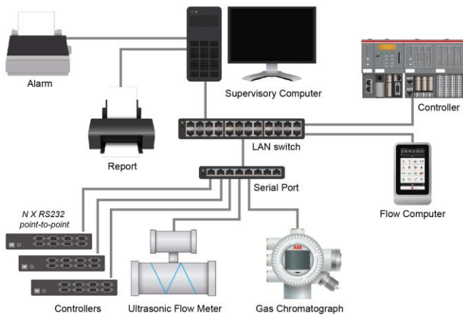
Figure 6.3 Point-to-point communications
