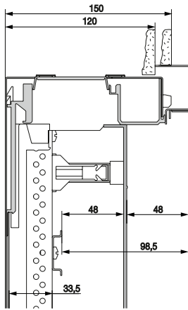
Distribution board panel
