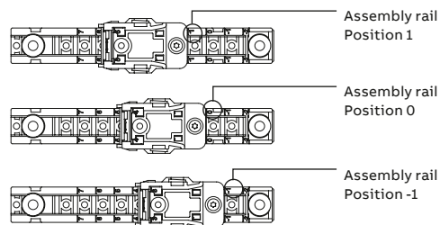
Assembly rail Top view
