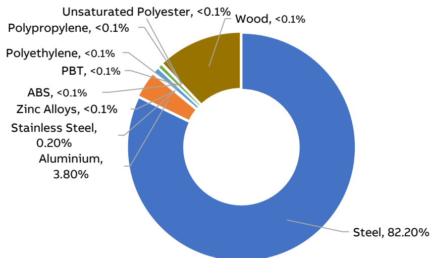
Figure 1: Composition of CDC640 Cabinet
