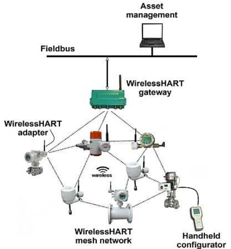
Figure 4. WirelessHART mesh network ensures system reliability.
